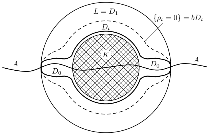
FIGURE 2. The sets D_t = \{\rho_t \leq 0\} .
