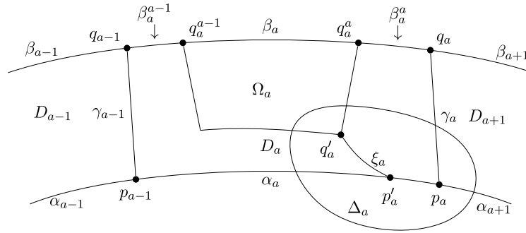
Fig. 1. Configuration of sets in X_j \setminus \dot{X}_{j-1} .
