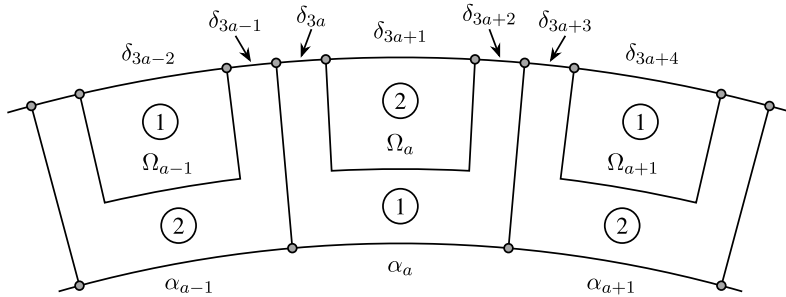
Fig. 2. The division \mathcal{D}^j of bX_j . Assuming that a \in \mathbb{Z}_l^{\text{odd}} , the numbers 1 and 2 inside the circles point out the component function u_{b,1}^j or u_{b,2}^j , respectively, that is suitably big in each set according to conditions (ii 5 ) to (ii 8 ).
