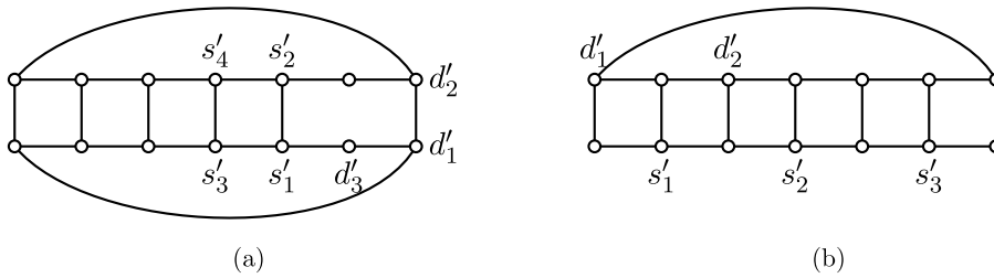
Fig. 4. Illustrating Staller's winning strategy in the proof of Proposition 4.5.
