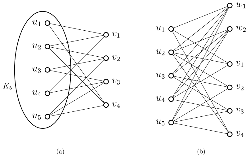
Fig. 6. The graph corresponding to the formula F following the constructions of the proof of Theorem 6.1 and of the proof of Corollary 6.2.
