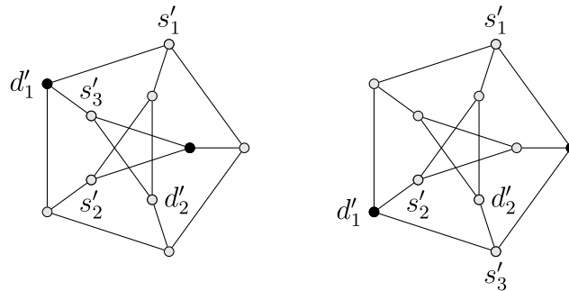
Fig. 2. The strategy of Staller in the S-game on P .
