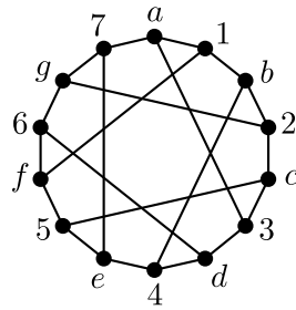
Fig. 1. The Heawood graph.
