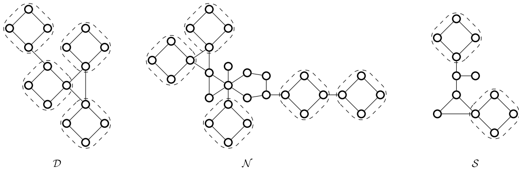
Fig. 5. Examples for each type of cactus.
