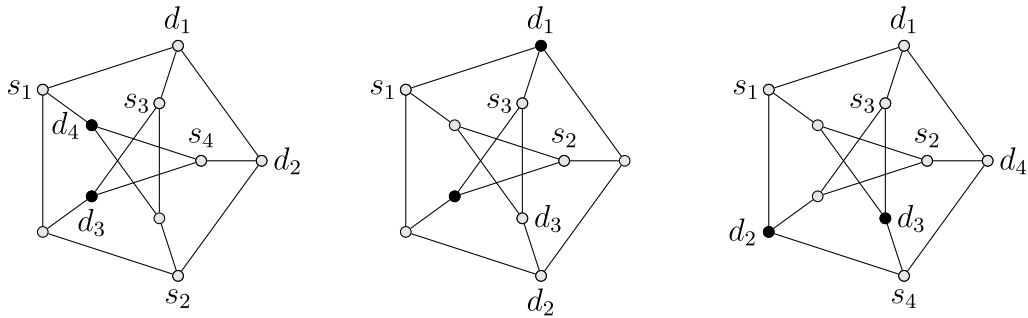
Fig. 3. The strategy of Staller in the D-game on P .
