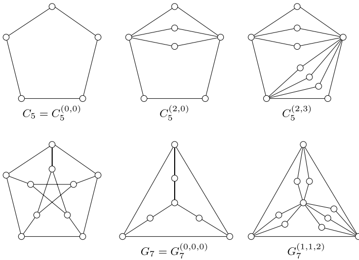
Fig. 3. Some examples of graphs from the family \mathcal{G} .
