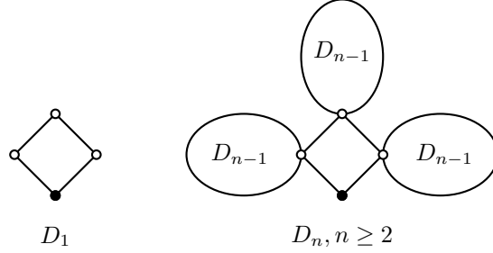
Figure 1: Recursive definition of the Bethe cacti D_n
