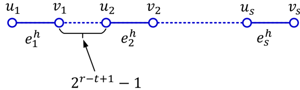
Figure 4: R^h = \{e_1^h, e_2^h, \dots, e_s^h\} . The vertices u_1, v_1, u_2, v_2, \dots, u_s, v_s are in increasing order. Also, d(e_i^h, e_{i+1}^h) \geq 2^{r-t+1} - 1 .
