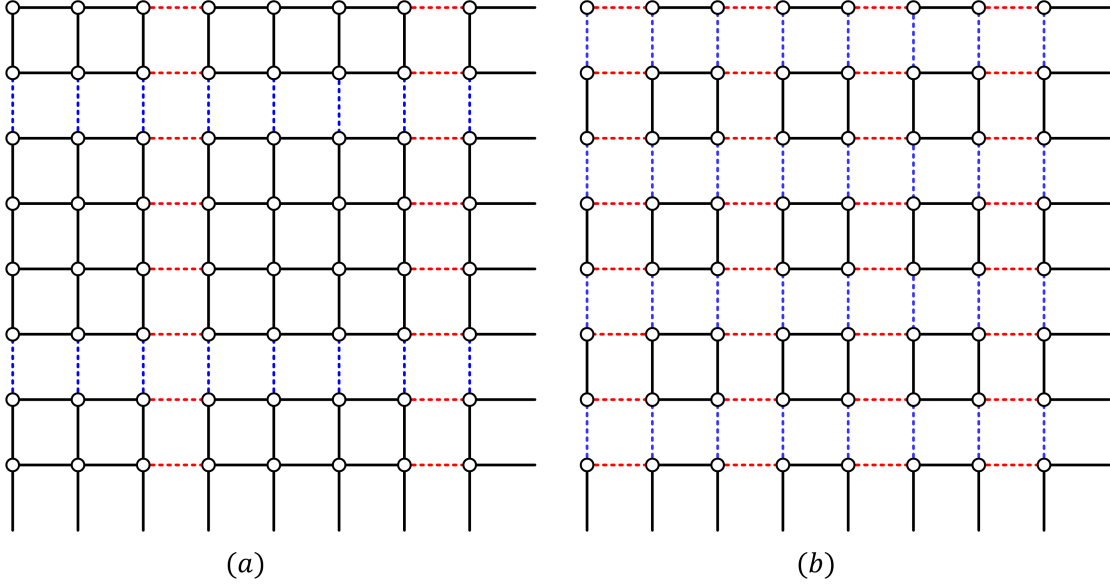
Figure 3: There are two type of edges: red dotted edges and blue dotted edges. The blue dotted edges are vertical and the red dotted edges are horizontal. (a) The red dotted edges and the blue dotted edges form an edge 3-general position set of the 8 \times 8 torus. (b) The red dotted edges and the blue dotted edges form an edge 5-general position set of the 8 \times 8 torus.
