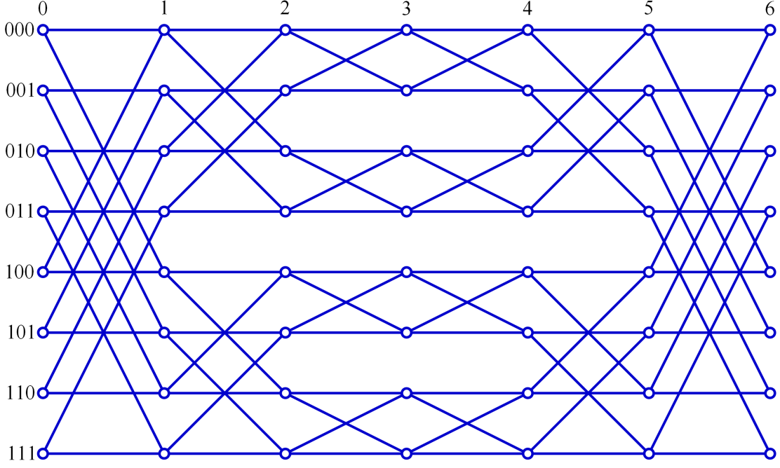
Figure 5: The Benes network BN(3) consists of back-to-back butterflies and is an edge disjoint union of two butterflies.
