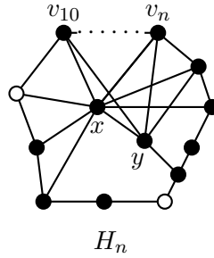
Figure 15: The graph H_n
