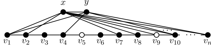
Figure 13: Graphs G_n
