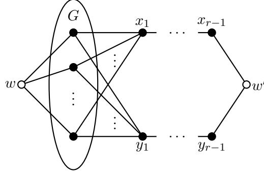
Figure 1: Graph \hat{G}_r
