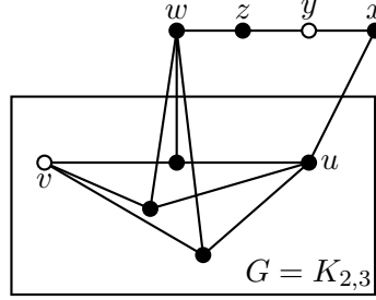
Figure 6: Graph H for G = K_{2,3}
