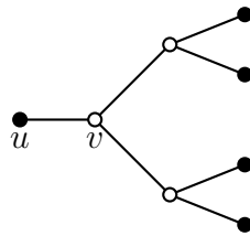
Figure 3: The tree T .
