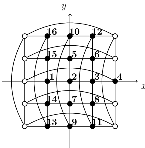
Figure 1: A dominating sequence of C_5 \square C_5
