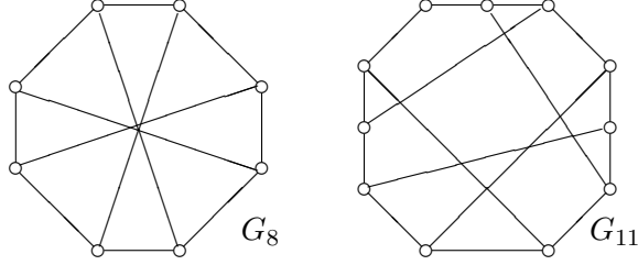
Figure 1: The graphs G_8 and G_{11}
