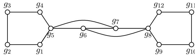
Figure 1. Graph G .
