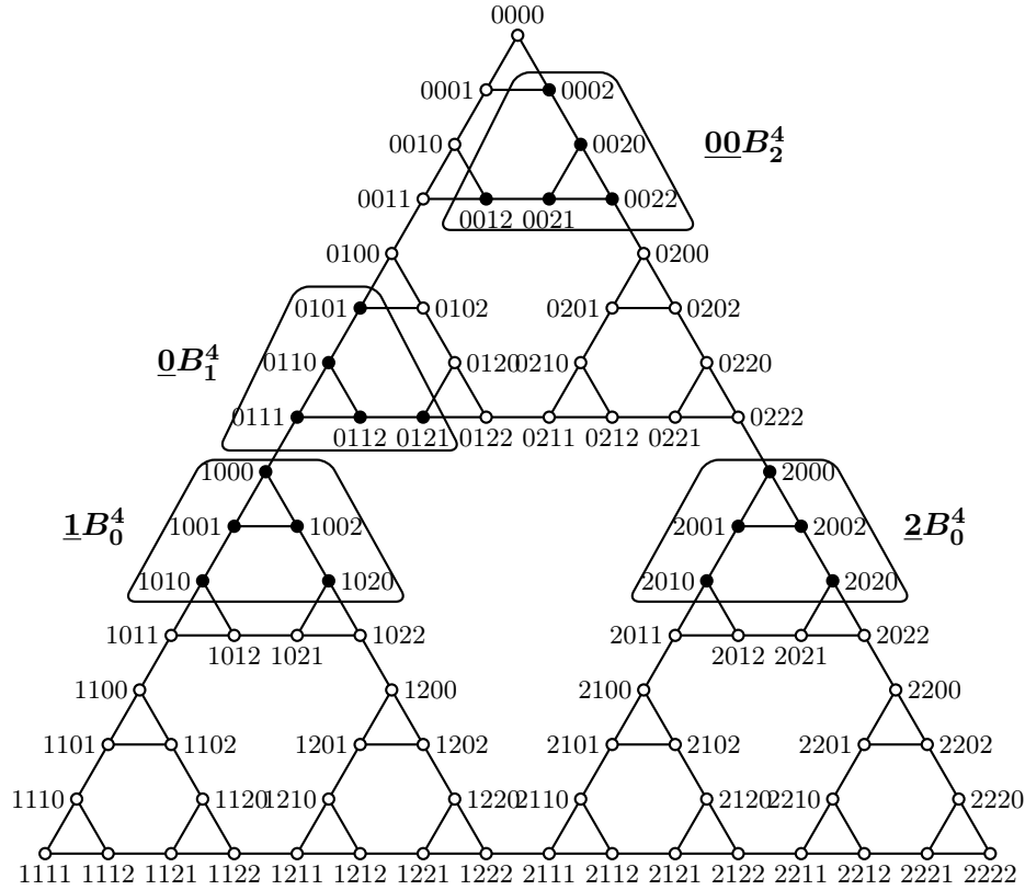
Figure 1. S_3^4 and some of its bulls.
