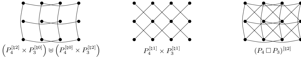
Figure 1: Illustration of the structure of (P_4 \square P_3)^{[2]} which is isomorphic to \left( P_4^{[2]} \times P_3^{[0]} \right) \uplus \left( P_4^{[0]} \times P_3^{[2]} \right) \uplus \left( P_4^{[1]} \times P_3^{[1]} \right) .
