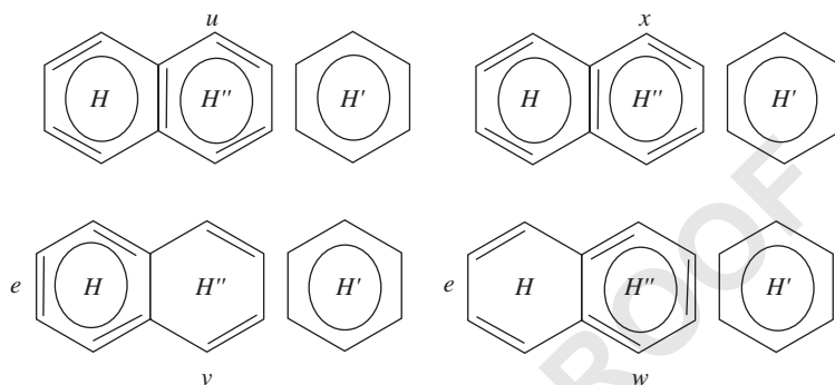
Fig. 2. One possible case of the hexagons H , H' and H'' are positioned relative to each other and the perfect matchings u , v , w , and x .
