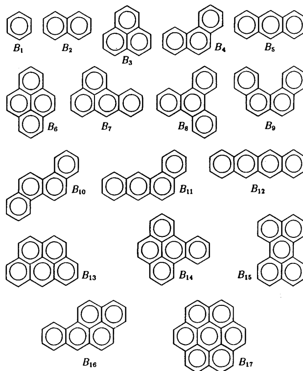
Figure 1. Some benzenoid systems.
