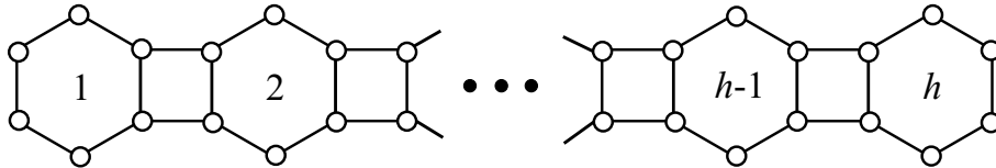
Figure 2: The linear phenylene P_h
