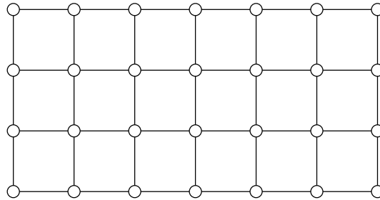
Figure 6: P_7 \square P_4
