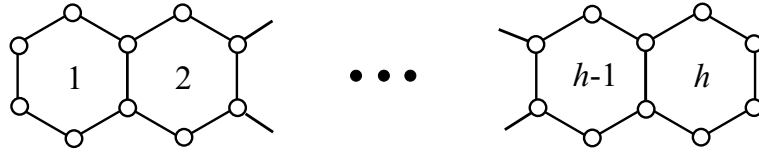
Figure 1: The linear chain L_h
