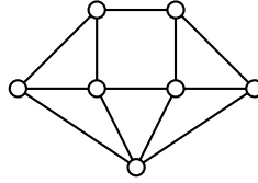
Figure 1. Graph G .
