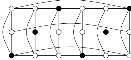
Figure 6: The set S in C_6 \square C_3 appears in bold.
