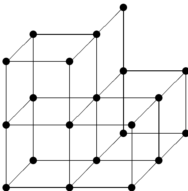
Figure 3: The resonance graph of fibonaccenes from the Figure 2.
