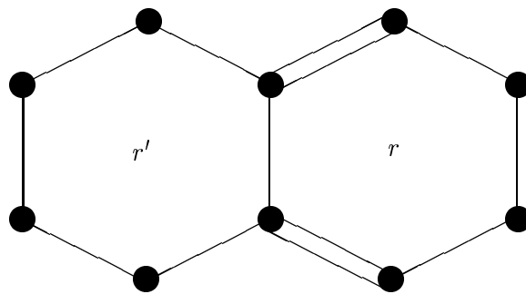
Figure 4: The link from r to r' .
