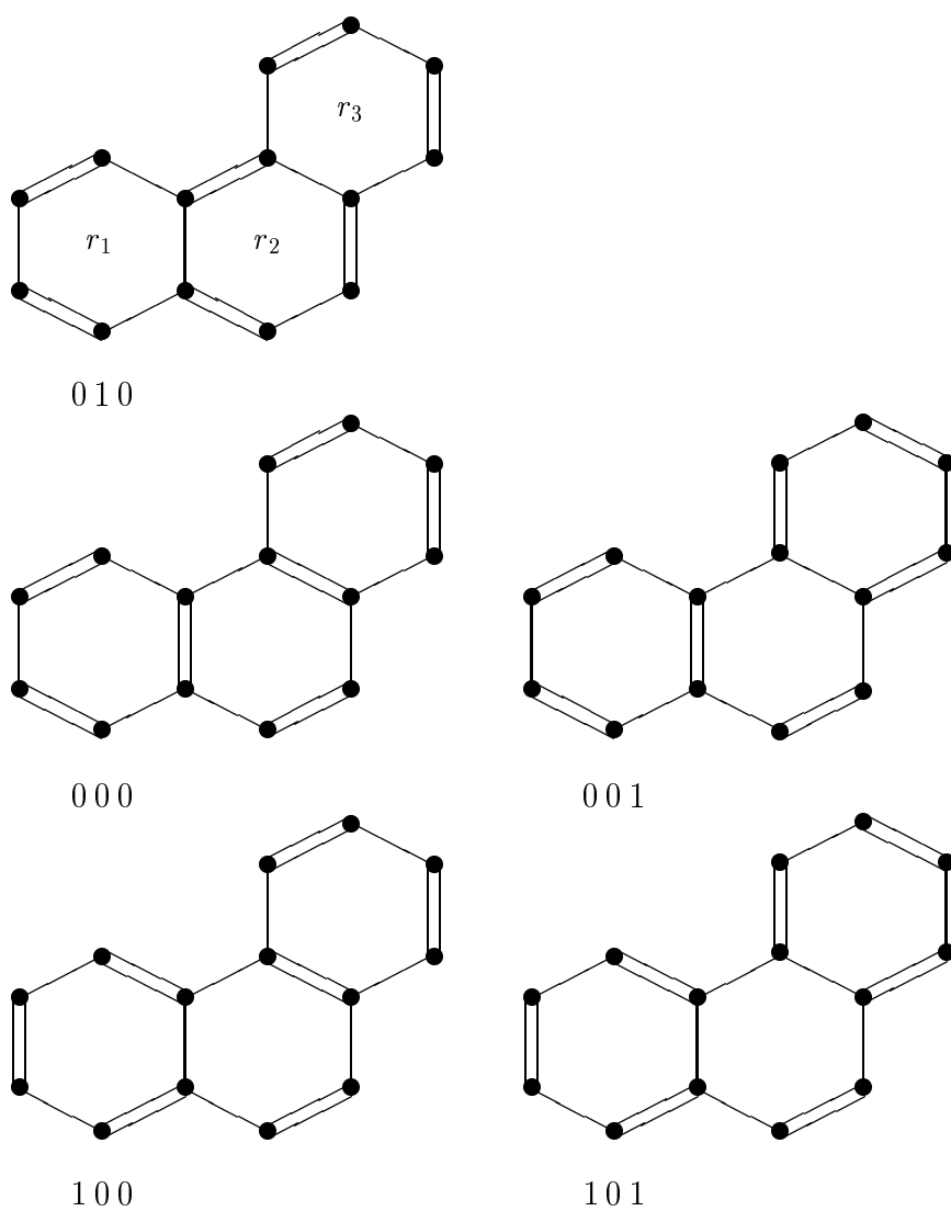
Figure 5: The labelings corresponding to the fibonaccene with three hexagons.
