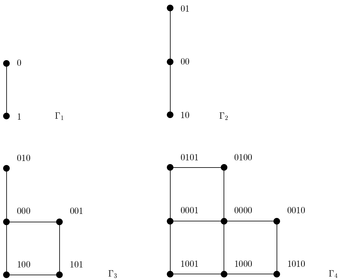
Figure 1: The first four Fibonacci cubes.
