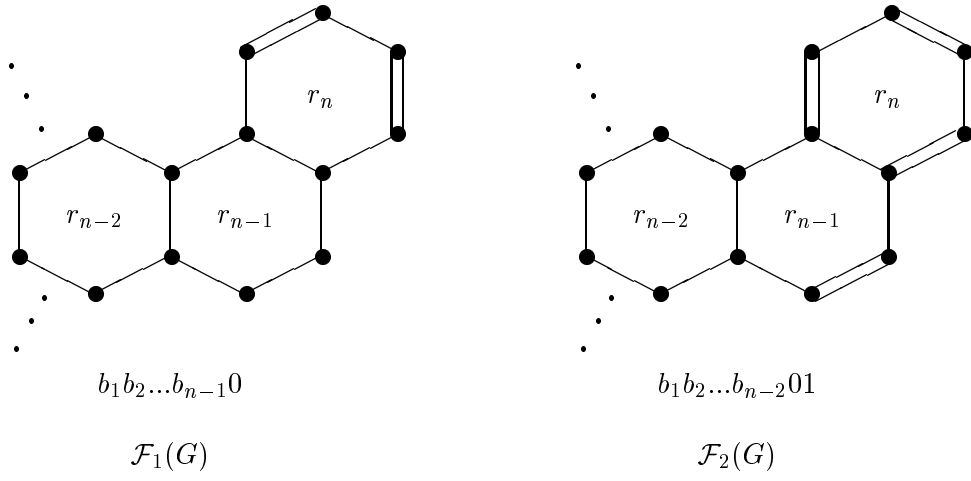
Figure 6: Fixed edges of 1-factors from \mathcal{F}_1(G) and \mathcal{F}_2(G) with associated labelings.
