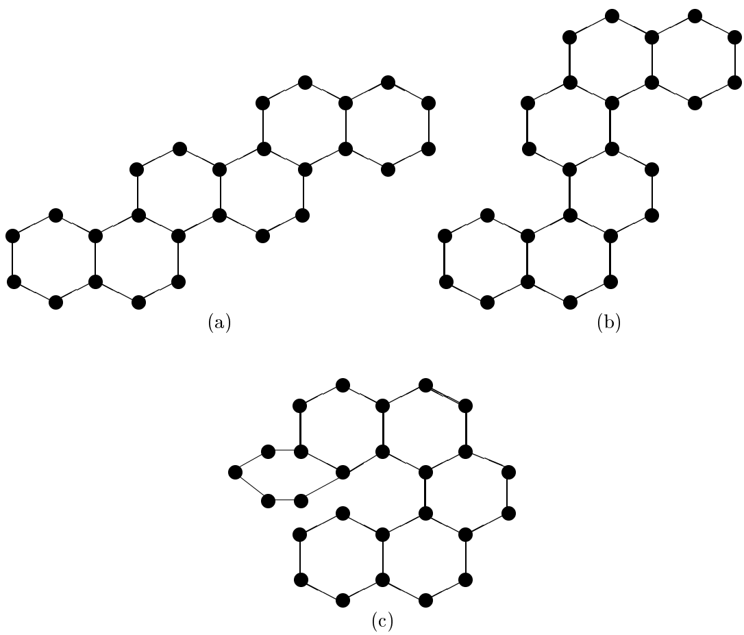
Figure 2: Some examples of fibonaccenes with six hexagons.
