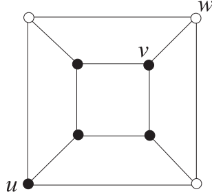
Figure 2: Example on antimedian.
