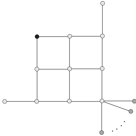
Figure 1: An antimedian vertex that is not peripheral.
