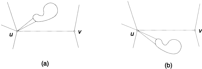
FIGURE 1. Change in the dual after a 2-switching
