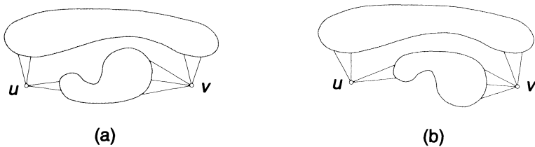
FIGURE 2. Local re-embedding of an \{x\} -component
