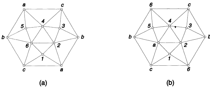
FIGURE 3. Triangulations of the projective plane
