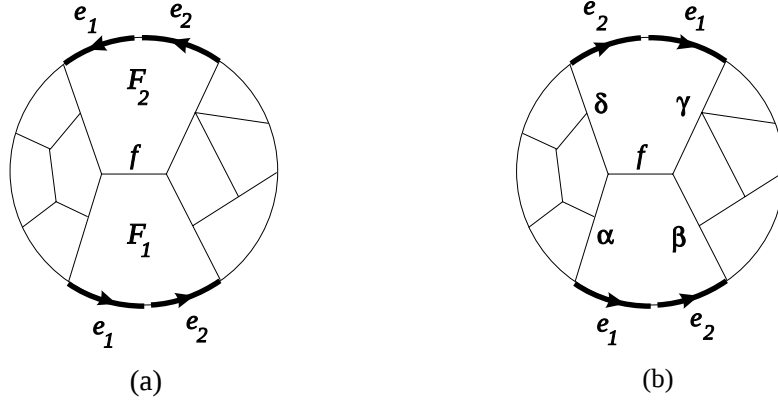
Figure 7: Pairs of singular branches of F
