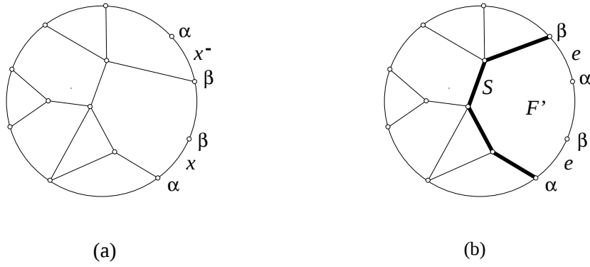
Figure 4: A singular branch on \partial F
