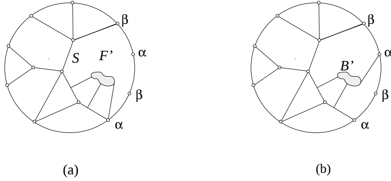
Figure 5: A bridge in F'
