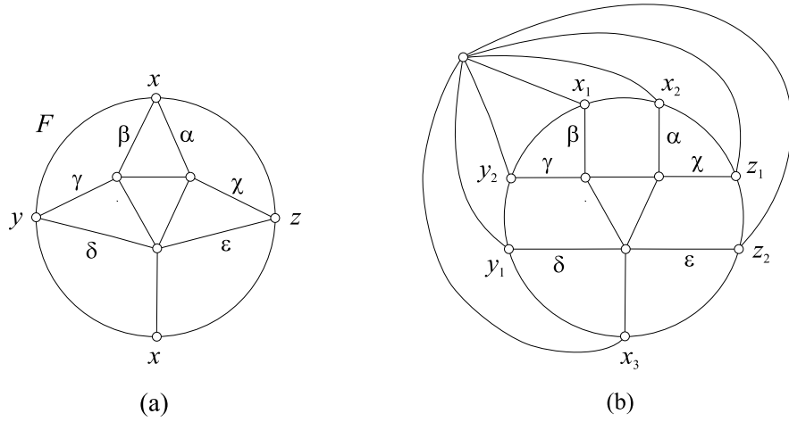
Figure 2: \Omega , \Pi , and \text{Aux}(\Omega, \Pi)
