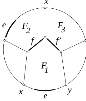
Figure 6: Overlapping of 2-embeddable bridges
