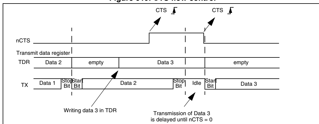
Figure 319. CTS flow control
