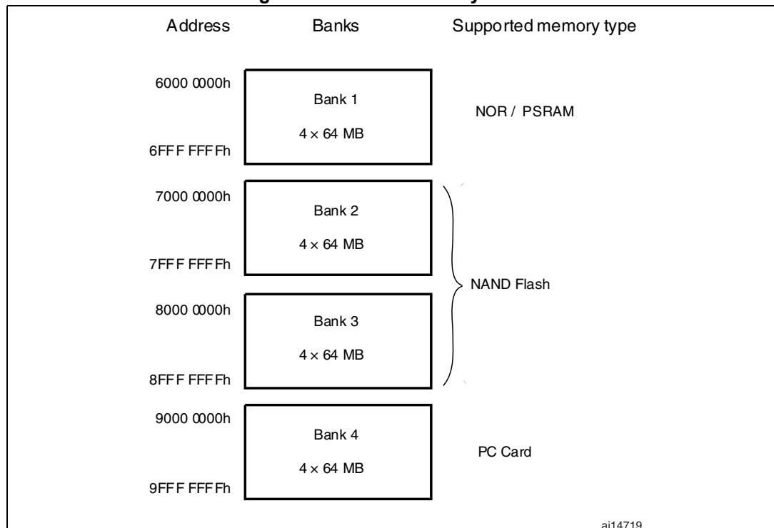
Figure 432. FSMC memory banks
