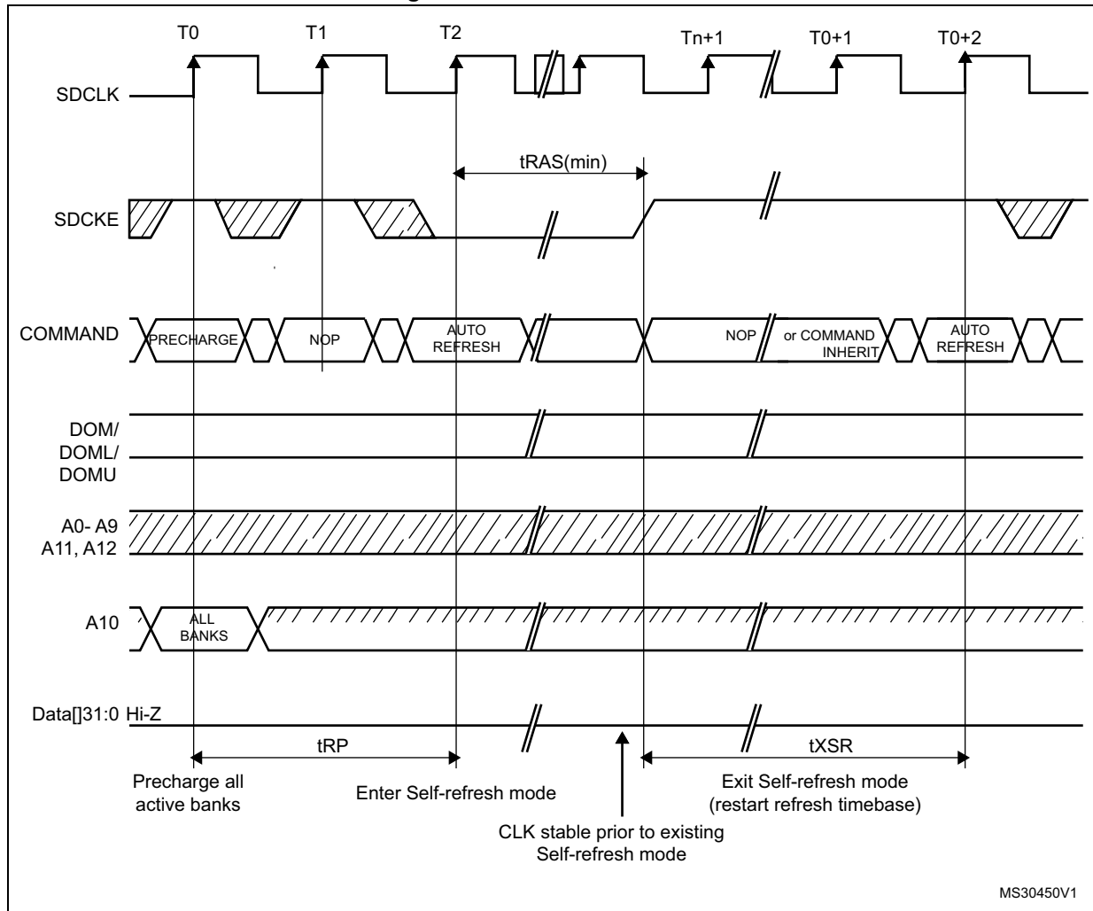
Figure 480. Self-refresh mode
