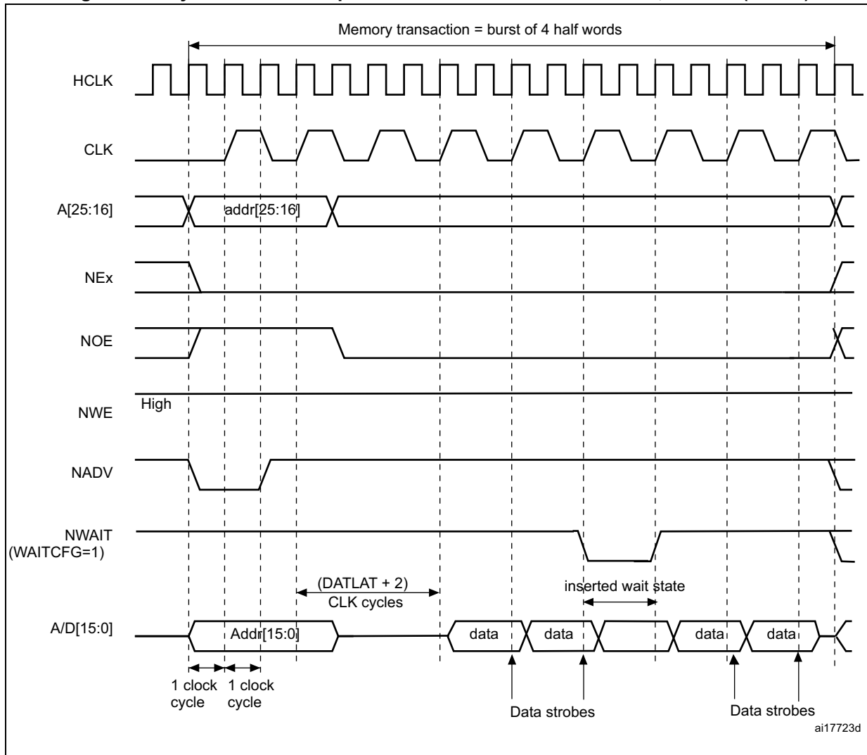
Figure 471. Synchronous multiplexed read mode waveforms - NOR, PSRAM (CRAM)
