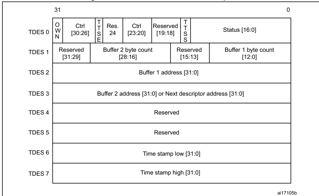
Figure 379. Enhanced transmit descriptor
