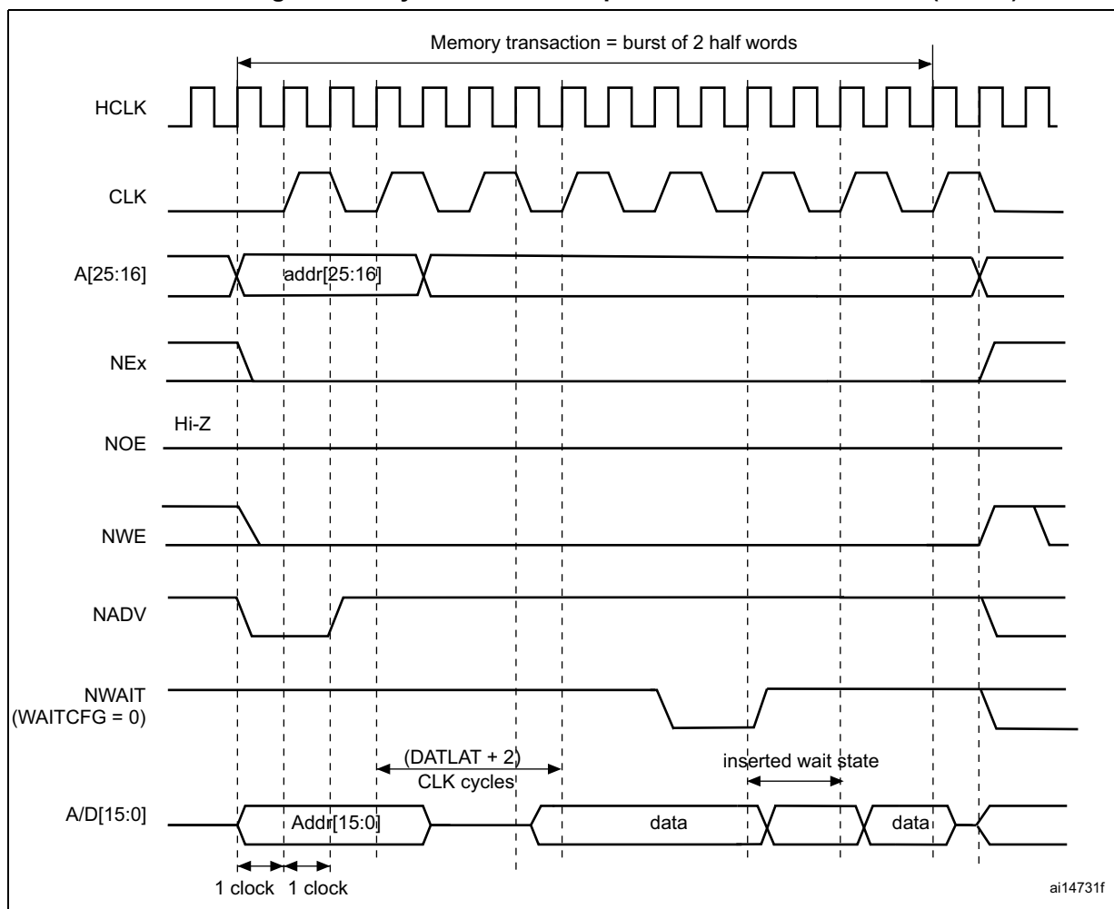
Figure 450. Synchronous multiplexed write mode - PSRAM (CRAM)
