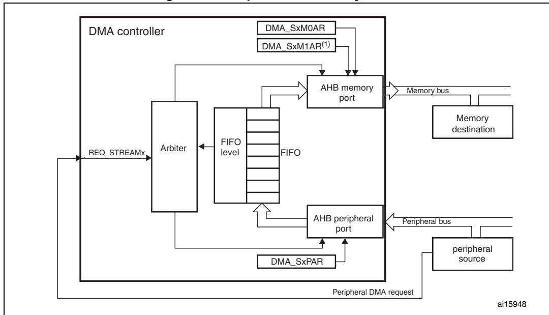
Figure 36. Peripheral-to-memory mode
