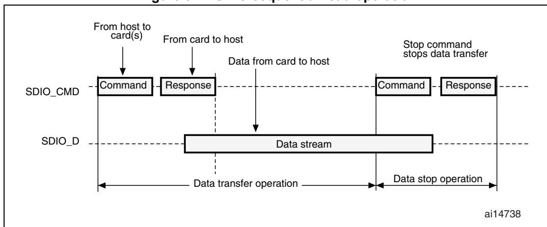
Figure 324. SDIO sequential read operation
