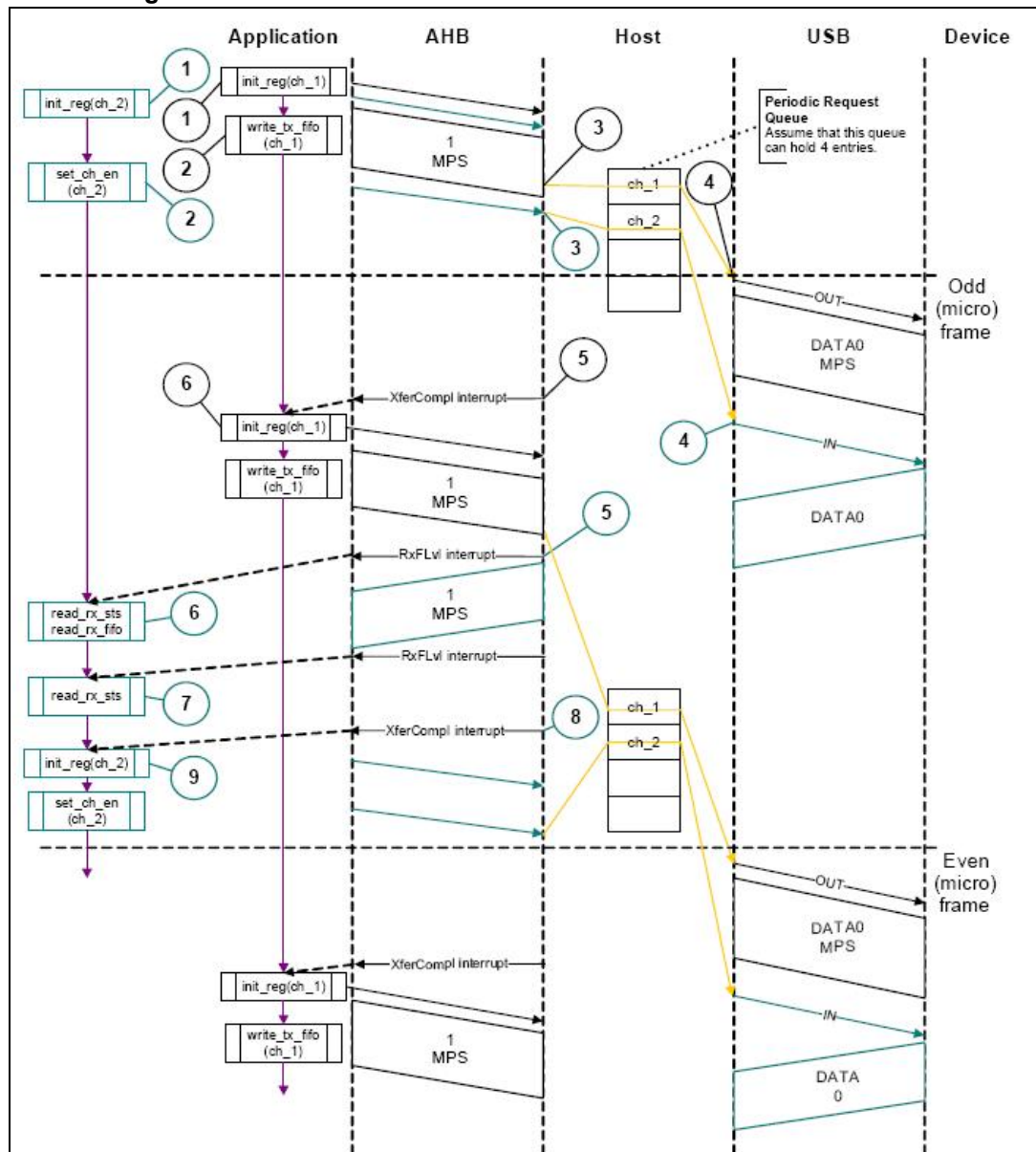
Figure 422. Normal isochronous OUT/IN transactions - Slave mode
