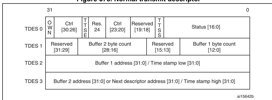
Figure 378. Normal transmit descriptor
