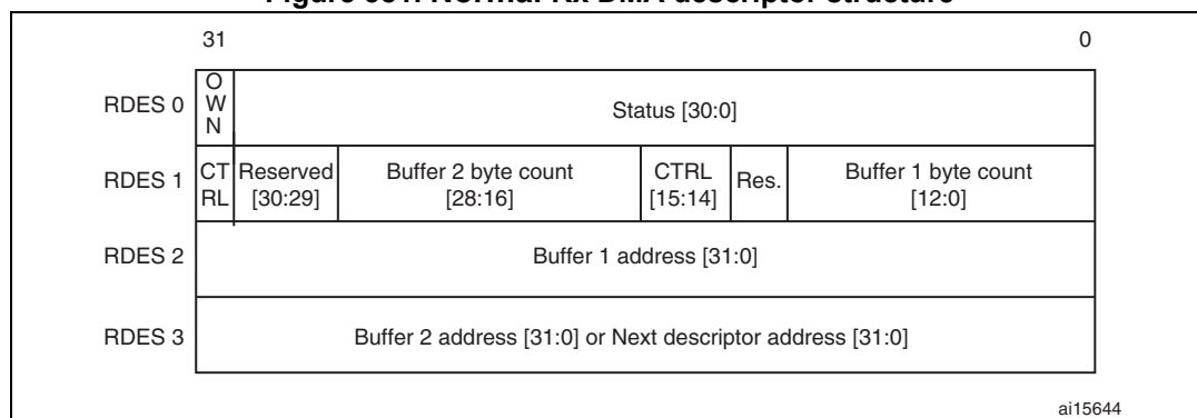
Figure 381. Normal Rx DMA descriptor structure
