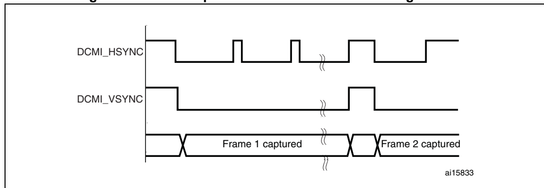
Figure 77. Frame capture waveforms in continuous grab mode
