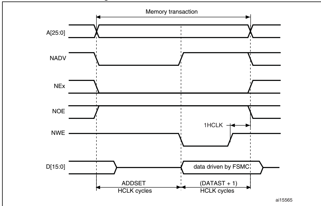
Figure 441. Mode C write accesses
