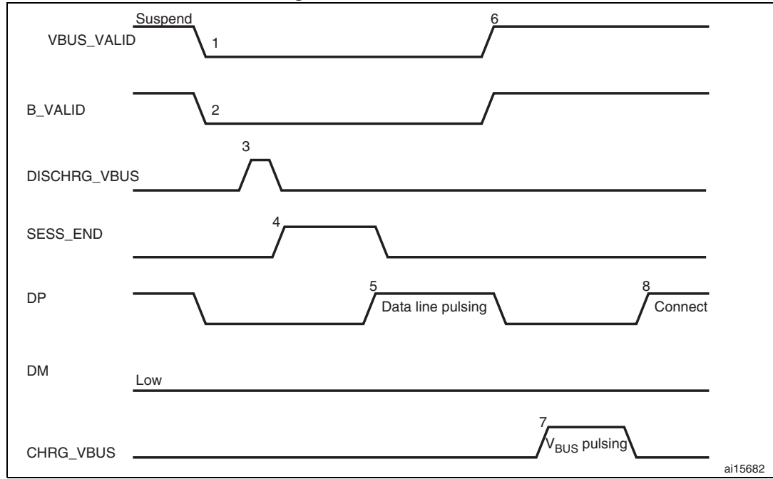
Figure 406. B-device SRP
