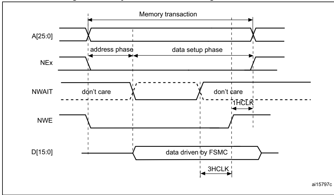
Figure 447. Asynchronous wait during a write access
