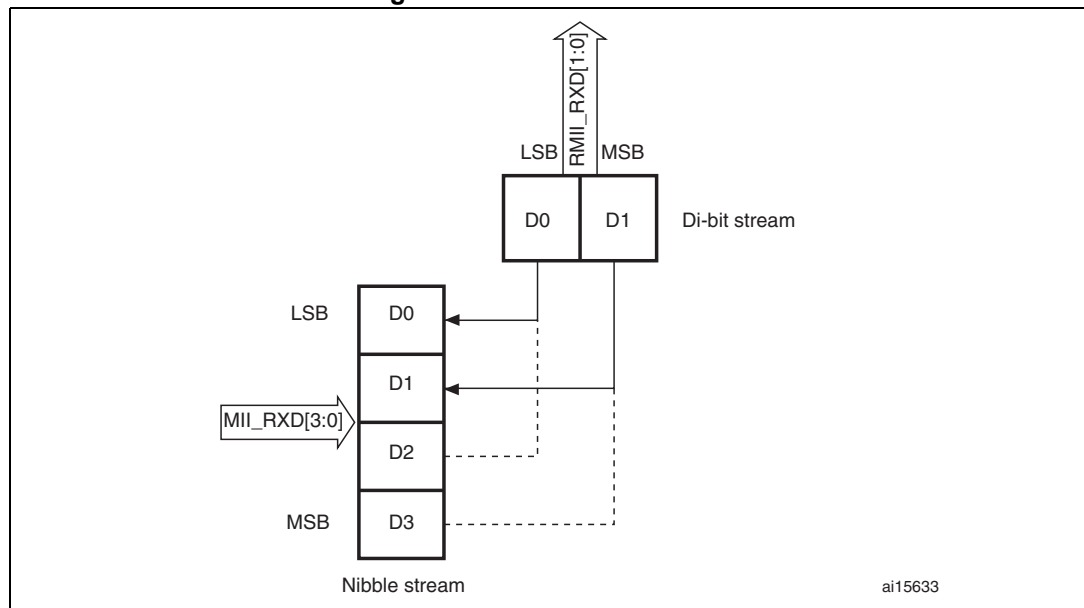
Figure 365. Receive bit order
