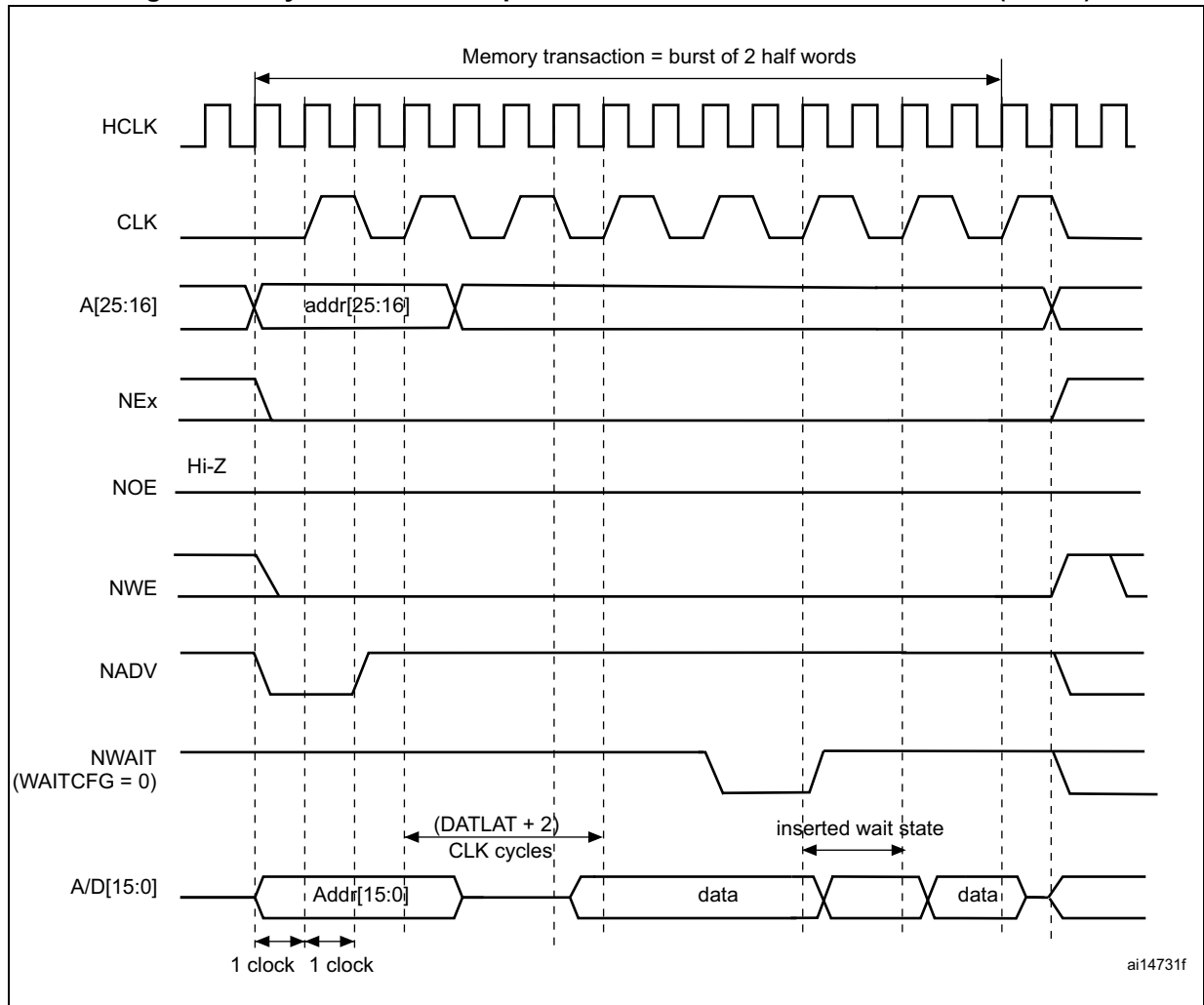
Figure 472. Synchronous multiplexed write mode waveforms - PSRAM (CRAM)
