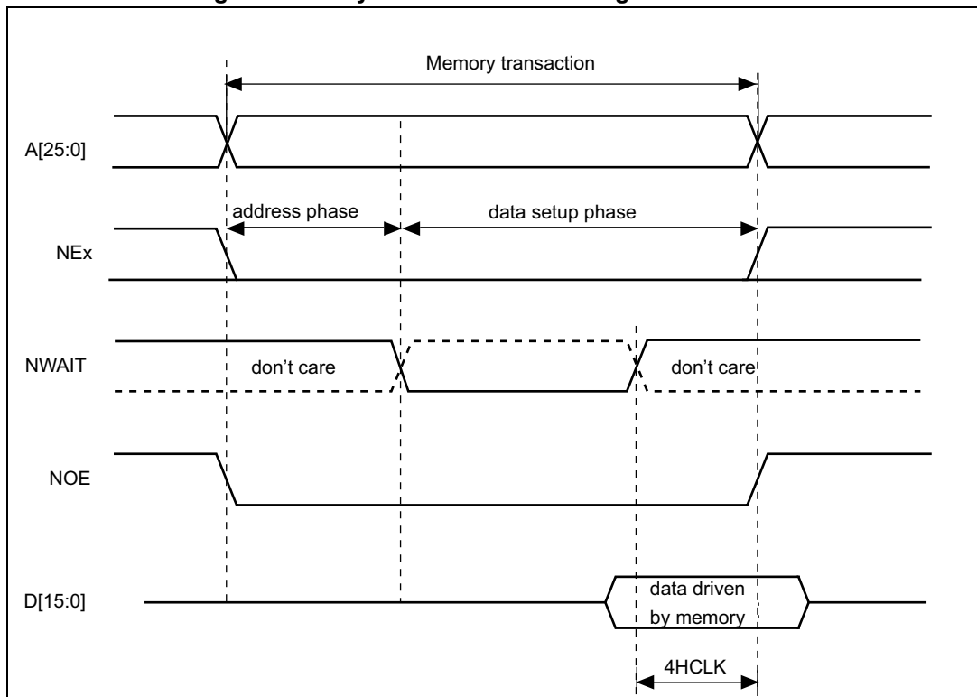
Figure 446. Asynchronous wait during a read access
