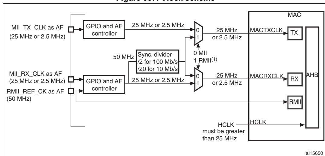
Figure 357. Clock scheme
