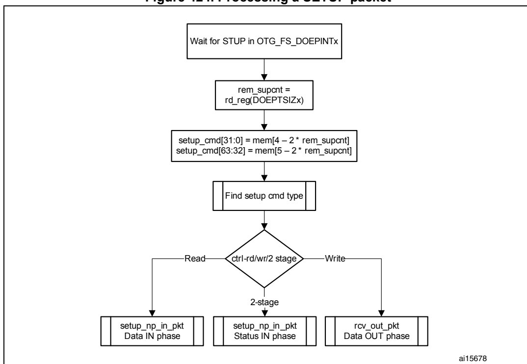
Figure 424. Processing a SETUP packet
