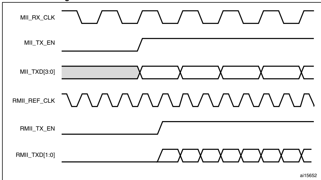
Figure 364. Frame transmission in MII and RMII modes
