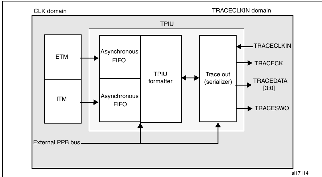
Figure 485. TPIU block diagram
