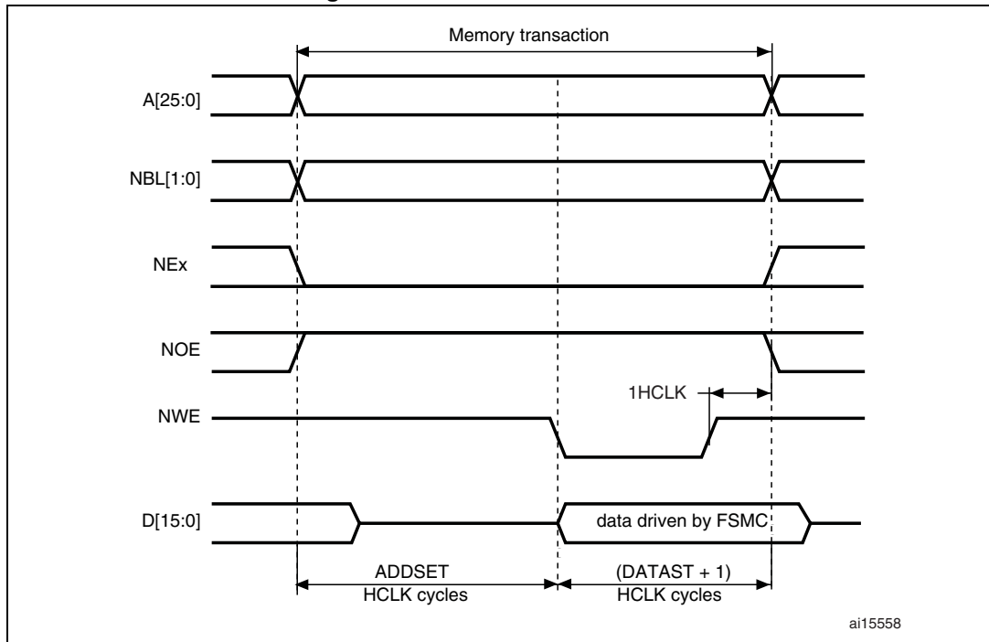
Figure 434. Mode1 write accesses
