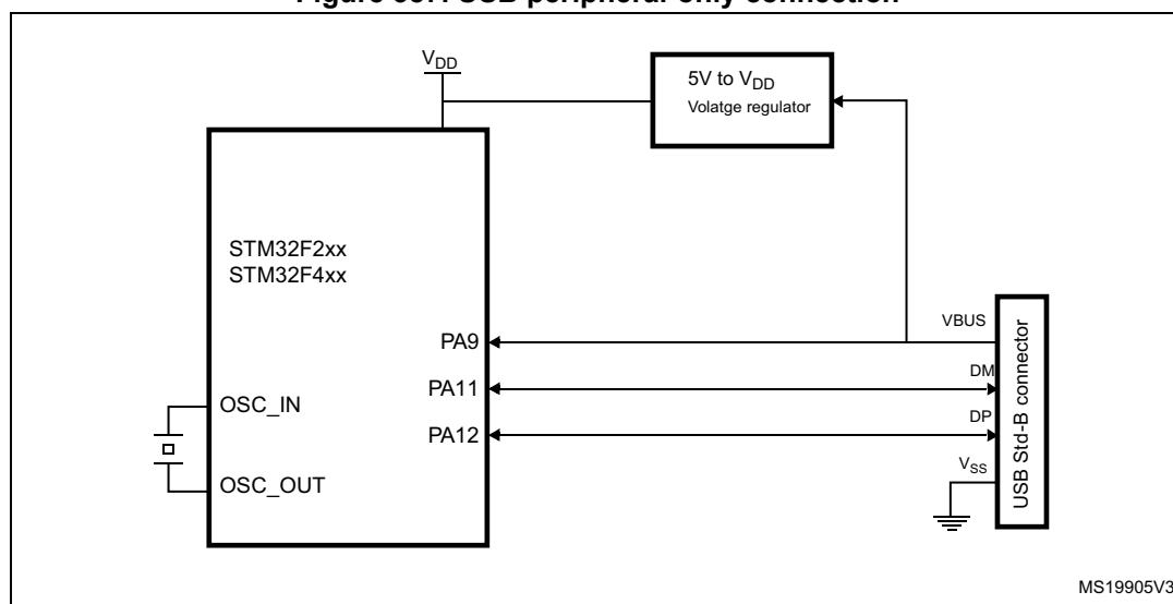
Figure 387. USB peripheral-only connection
