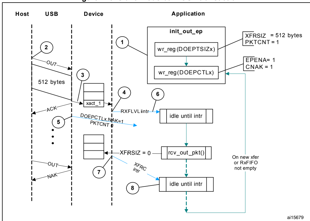
Figure 425. Slave mode bulk OUT transaction
