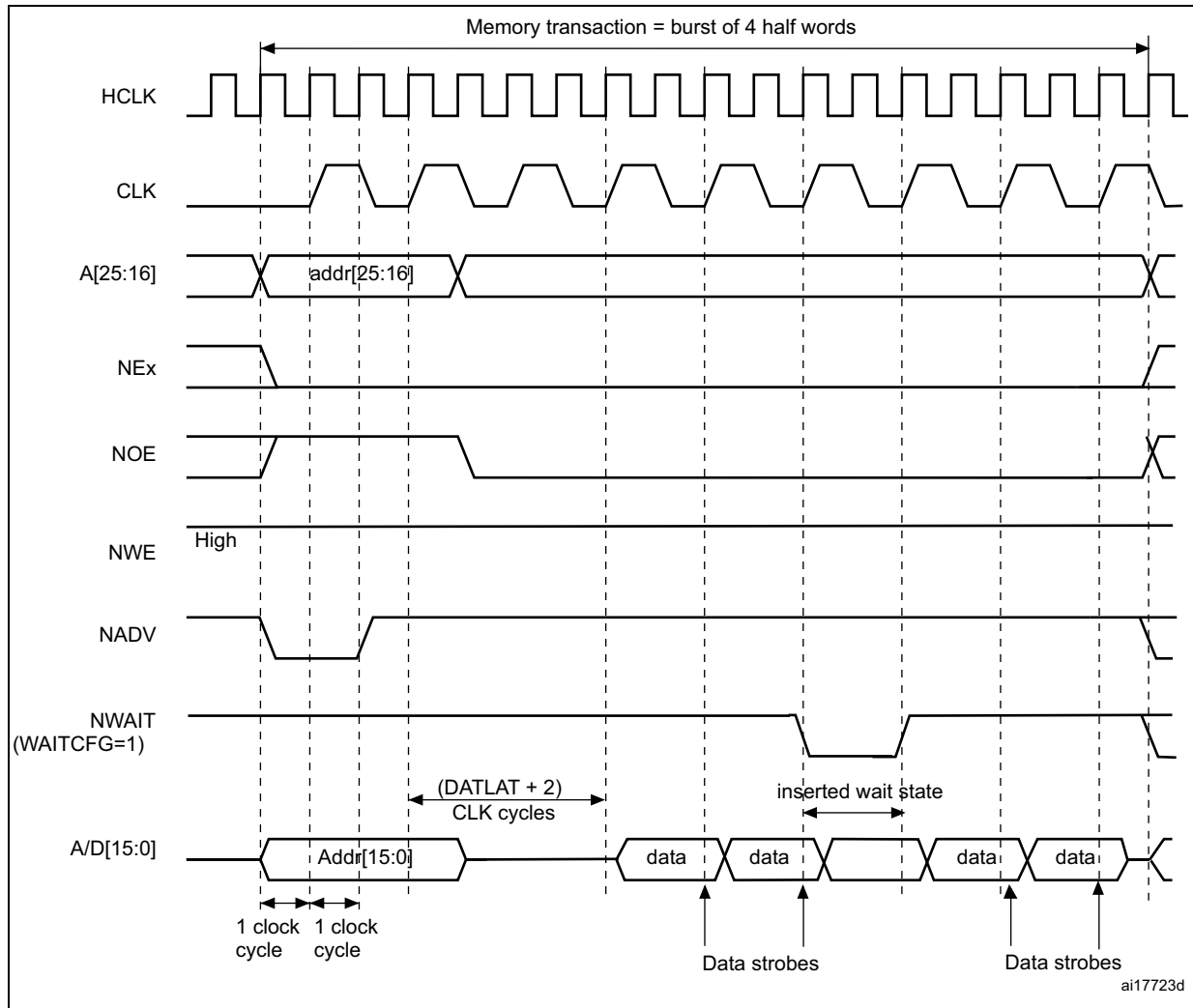
Figure 449. Synchronous multiplexed read mode - NOR, PSRAM (CRAM)
