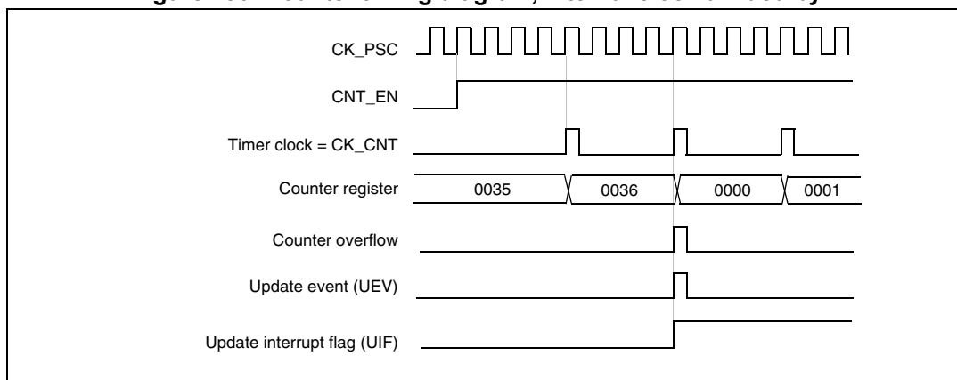
Figure 187. Counter timing diagram, internal clock divided by N
