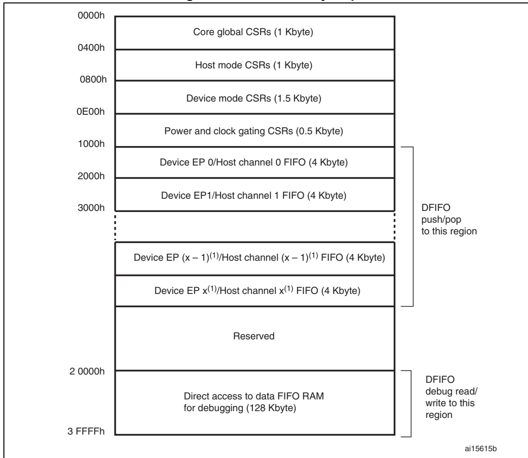
Figure 394. CSR memory map
