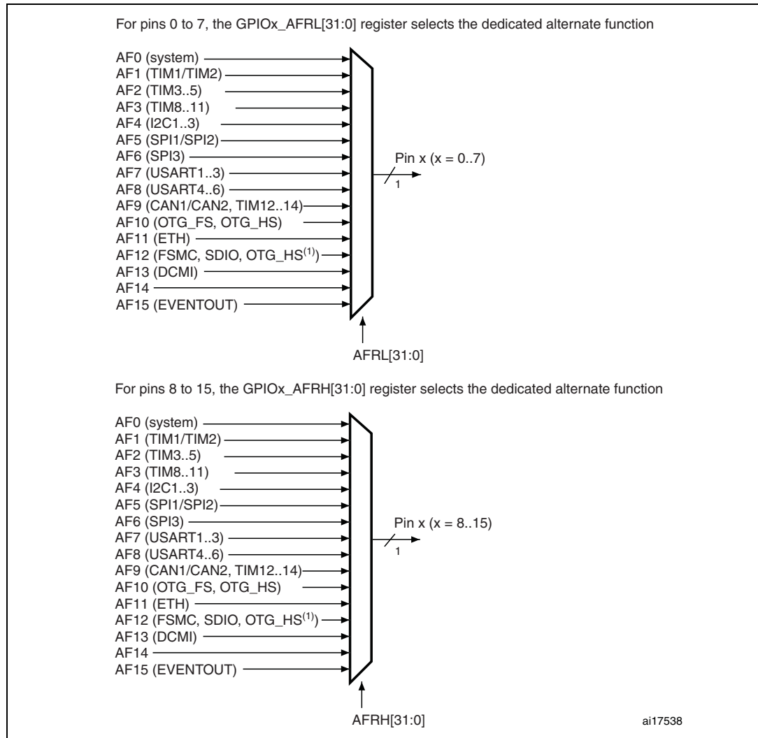
Figure 26. Selecting an alternate function on STM32F405xx/07xx and STM32F415xx/17xx
