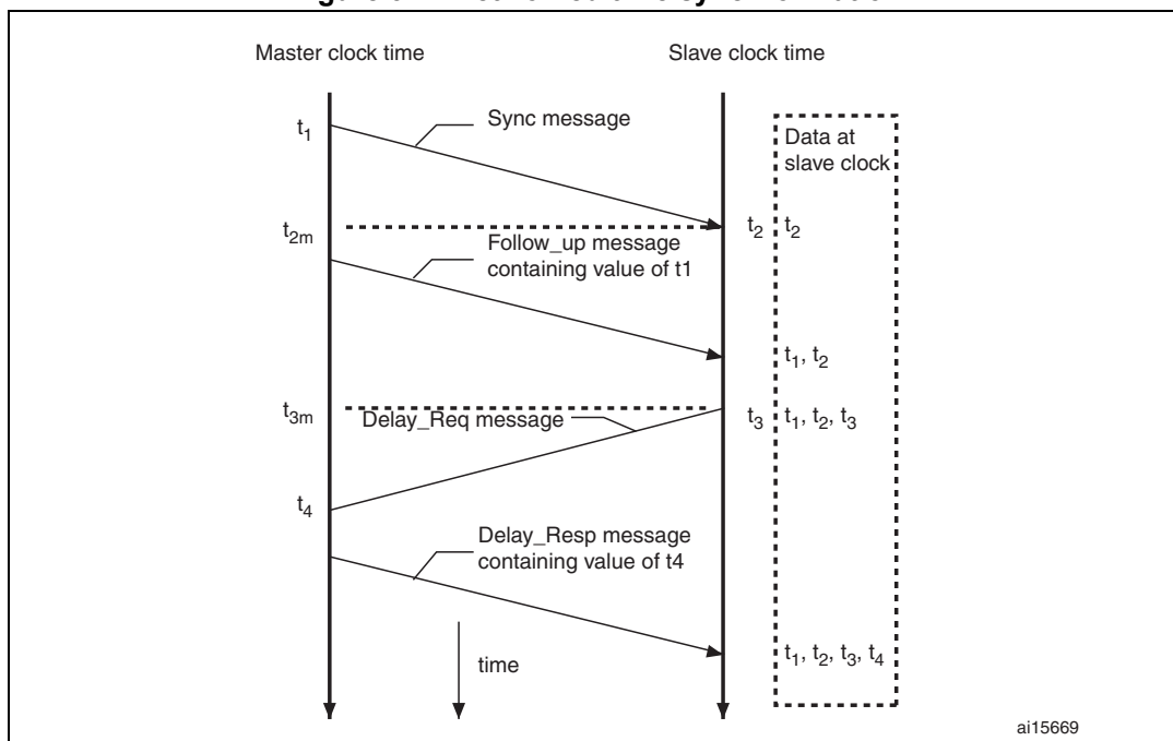
Figure 371. Networked time synchronization
