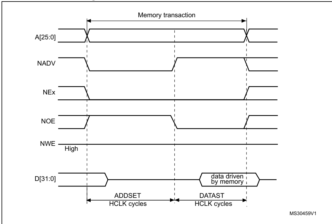
Figure 462. ModeC read access waveforms
