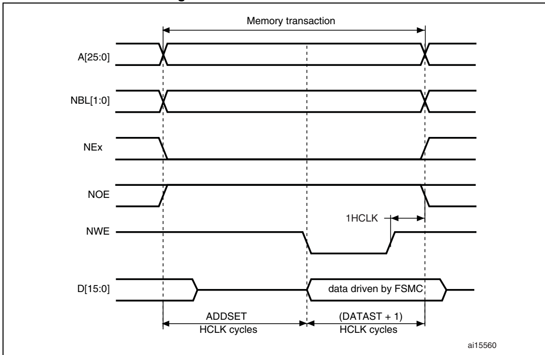
Figure 436. ModeA write accesses
