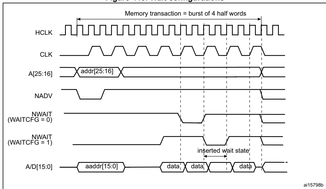
Figure 448. Wait configurations
