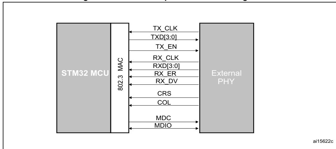
Figure 353. Media independent interface signals
