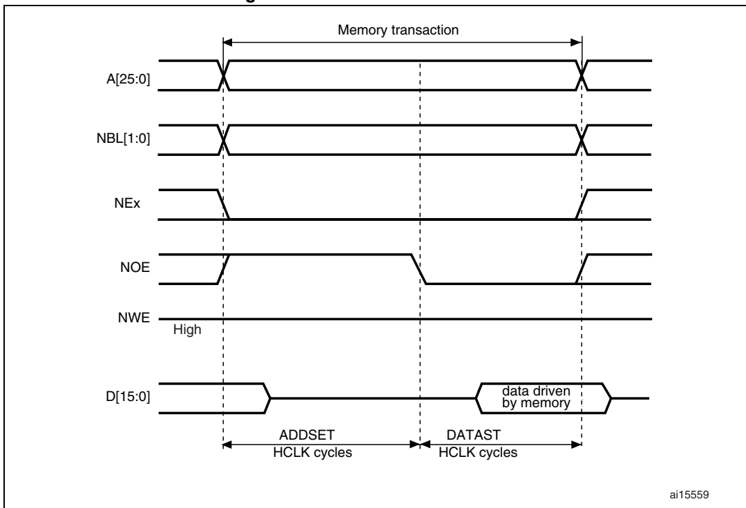
Figure 435. ModeA read accesses
