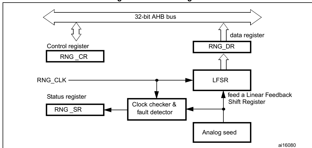
Figure 232. Block diagram
