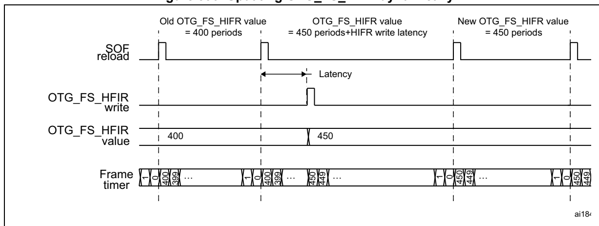
Figure 390. Updating OTG_FS_HFIR dynamically
