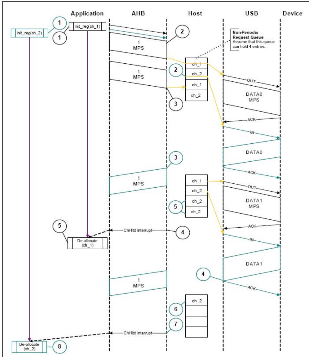
Figure 415. Normal bulk/control OUT/SETUP and bulk/control IN transactions - DMA mode
