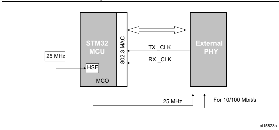
Figure 354. MII clock sources
