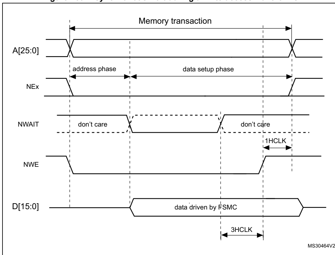
Figure 469. Asynchronous wait during a write access waveforms
