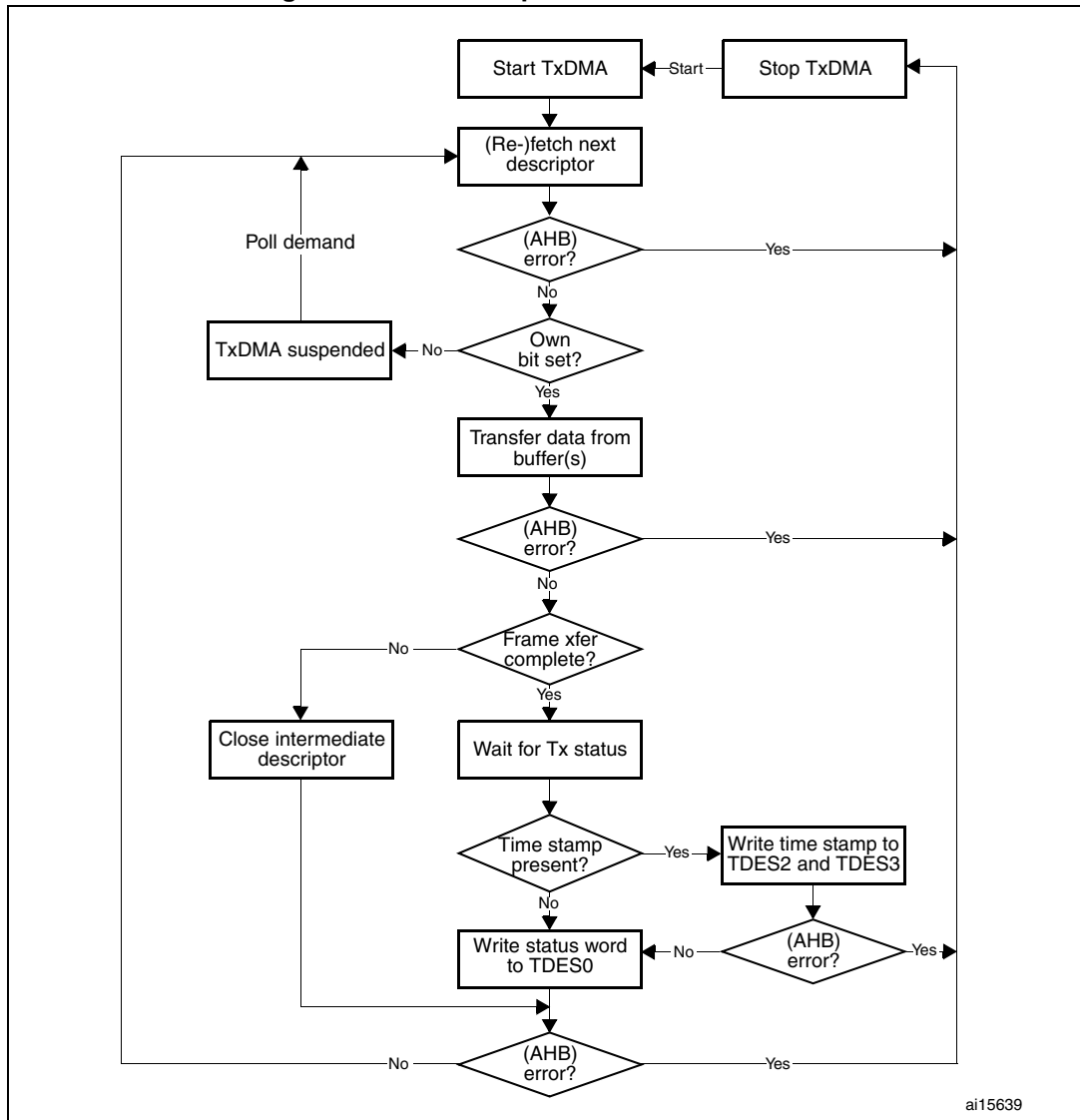
Figure 376. TxDMA operation in Default mode
