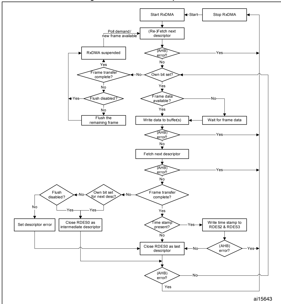
Figure 380. Receive DMA operation
