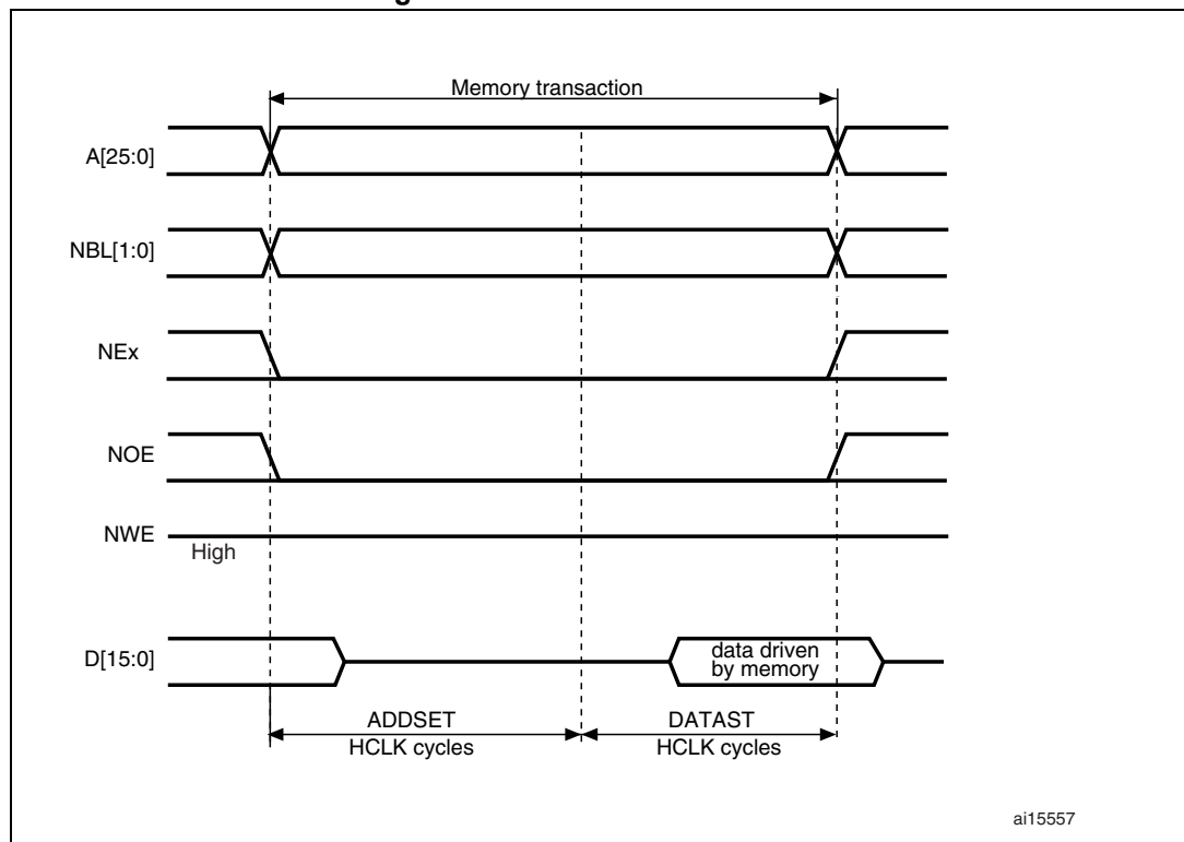
Figure 433. Mode1 read accesses
