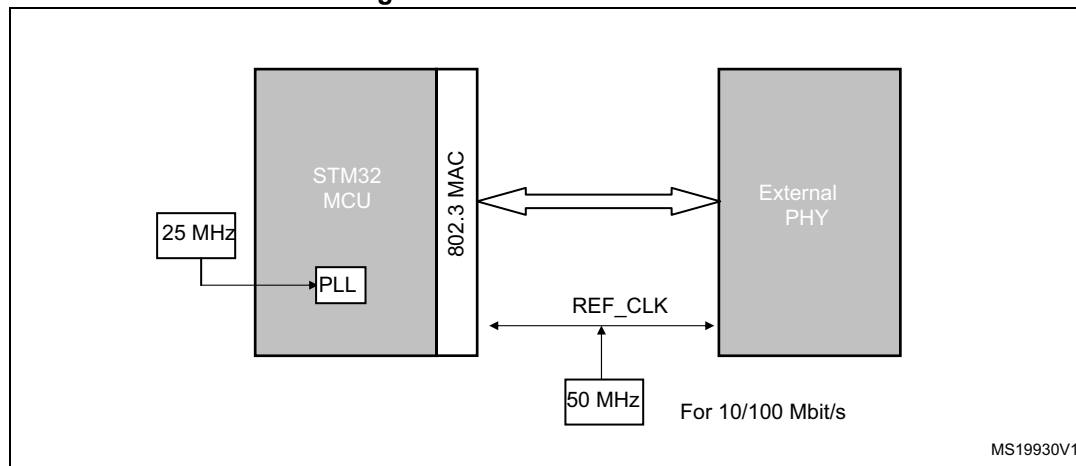
Figure 356. RMII clock sources
