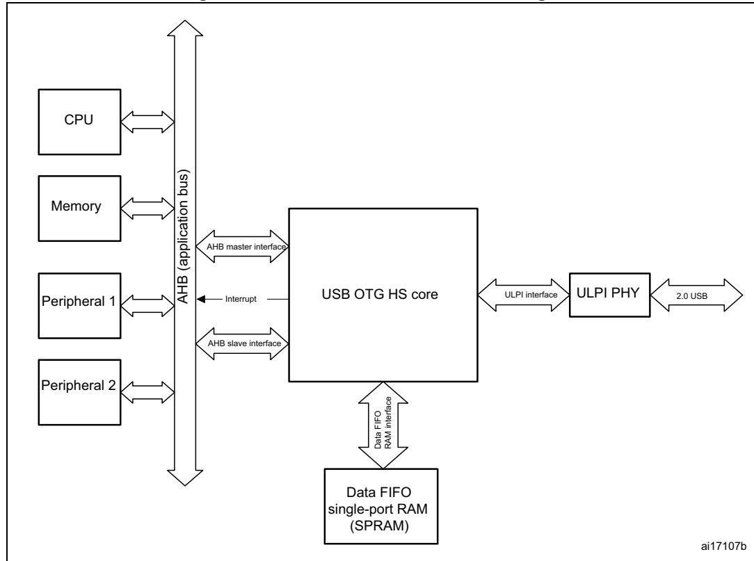
Figure 409. USB OTG interface block diagram
