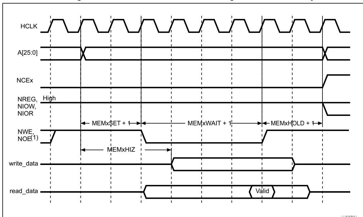
Figure 451. NAND/PC Card controller timing for common memory access
