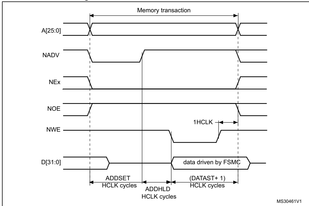
Figure 465. ModeD write access waveforms
