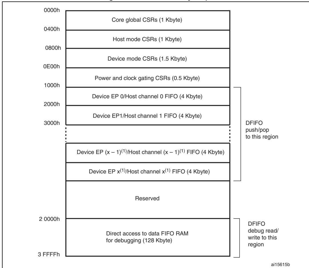
Figure 412. CSR memory map
