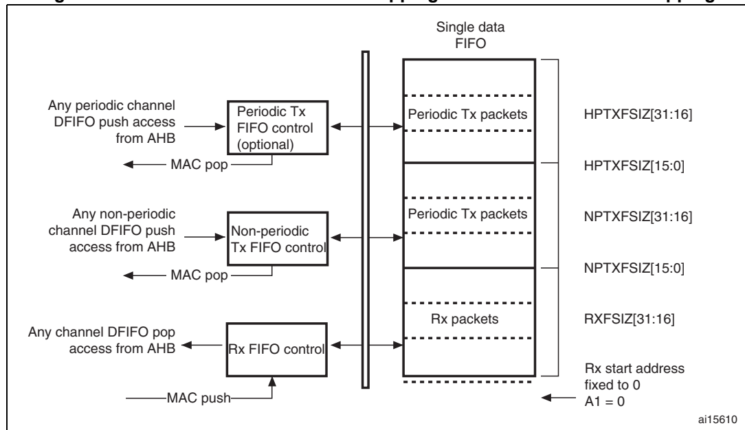
Figure 392. Host-mode FIFO address mapping and AHB FIFO access mapping
