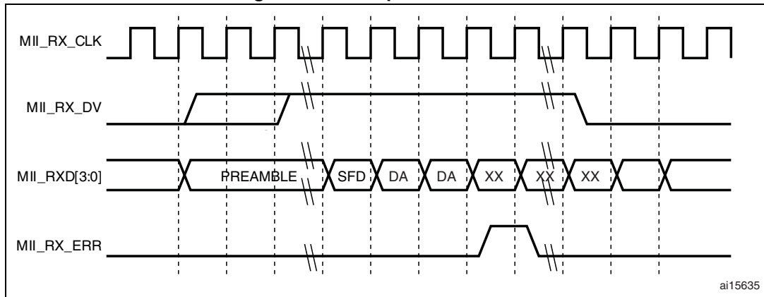
Figure 367. Reception with errors
