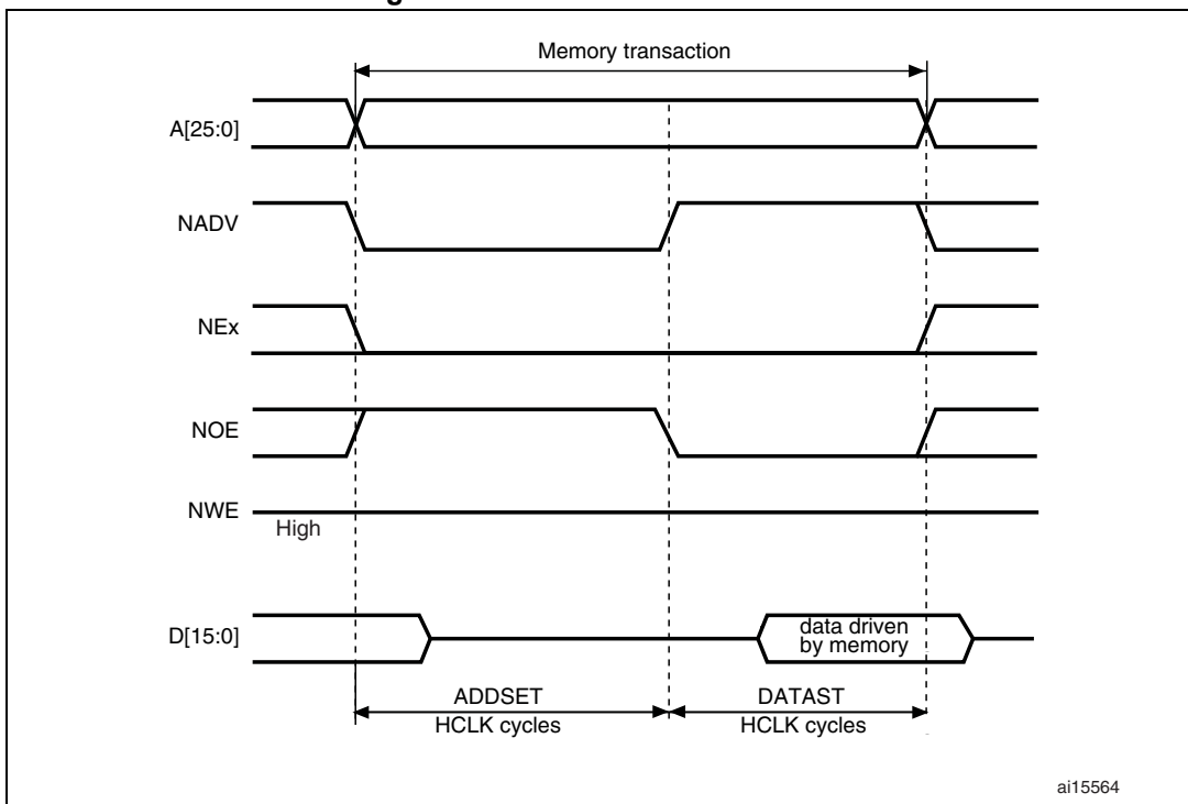
Figure 440. Mode C read accesses
