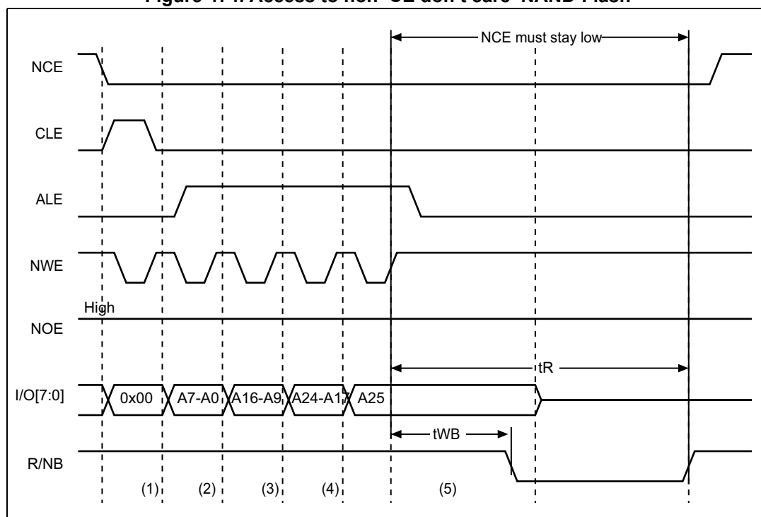
Figure 474. Access to non ‘CE don’t care’ NAND-Flash
