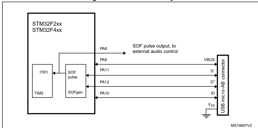
Figure 389. SOF connectivity
