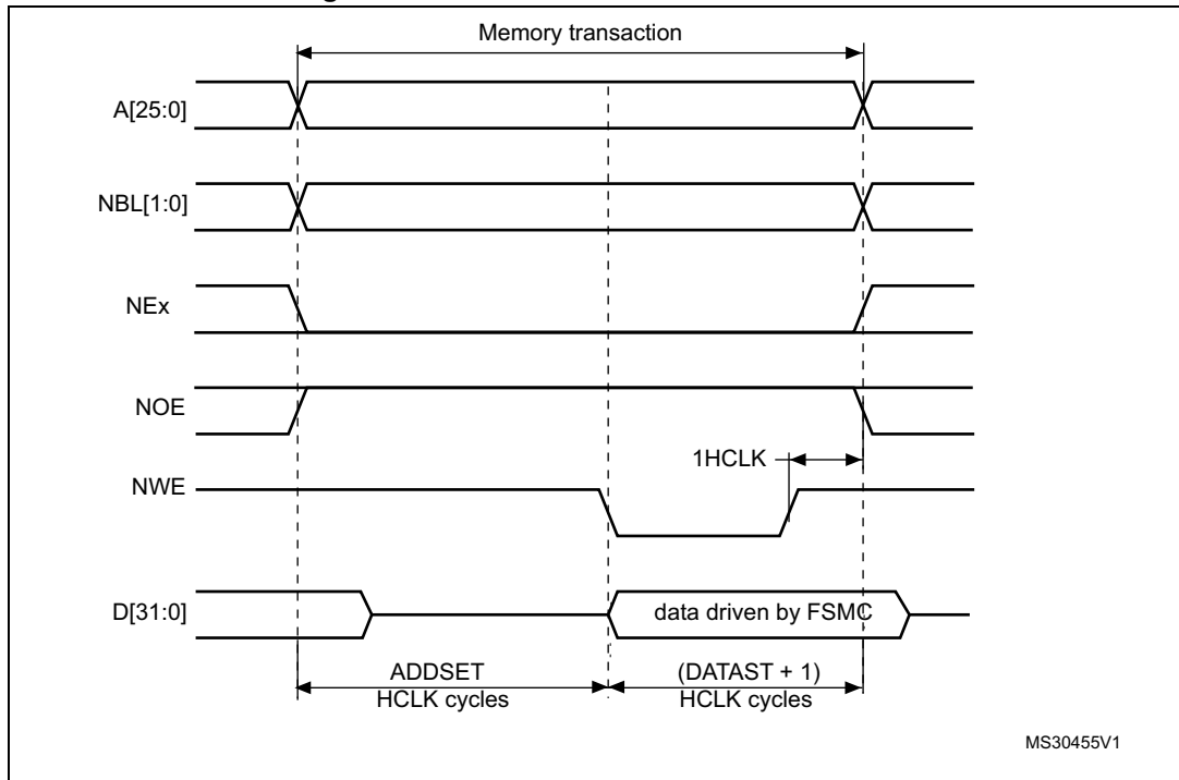
Figure 458. ModeA write access waveforms
