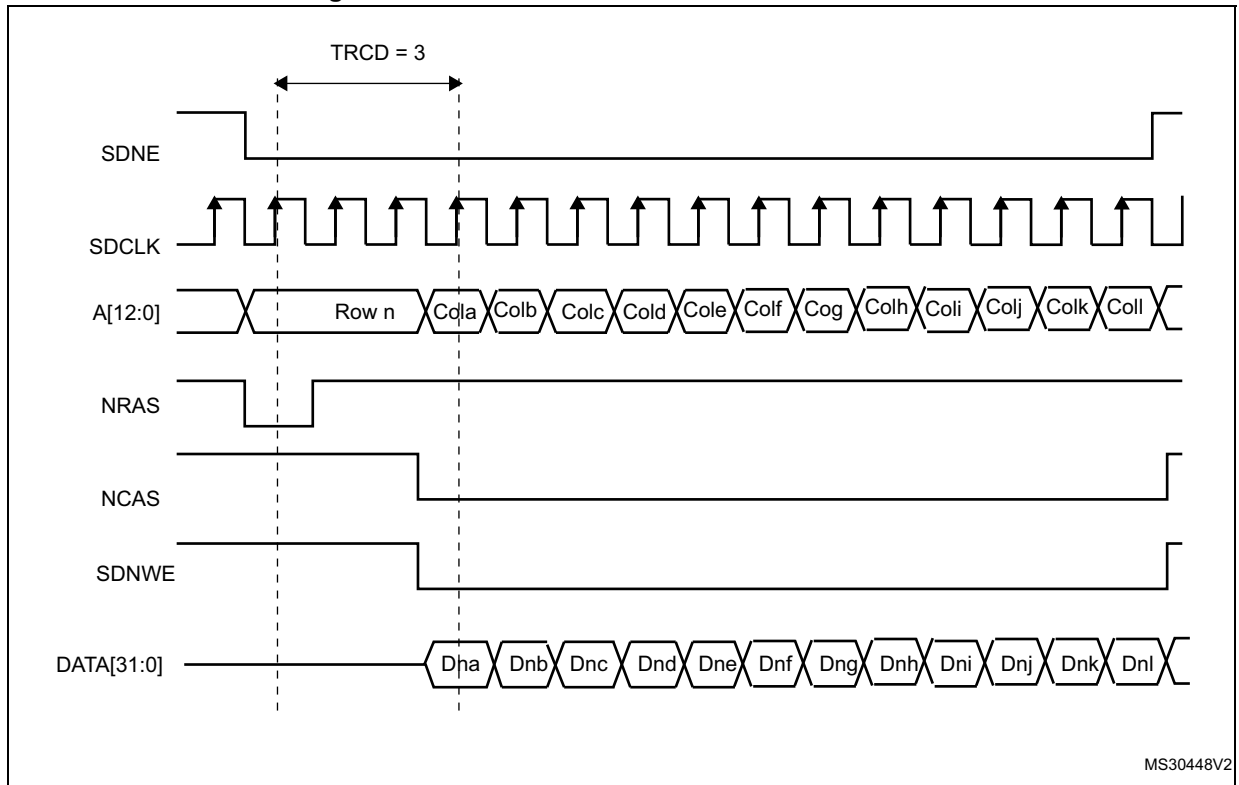
Figure 475. Burst write SDRAM access waveforms
