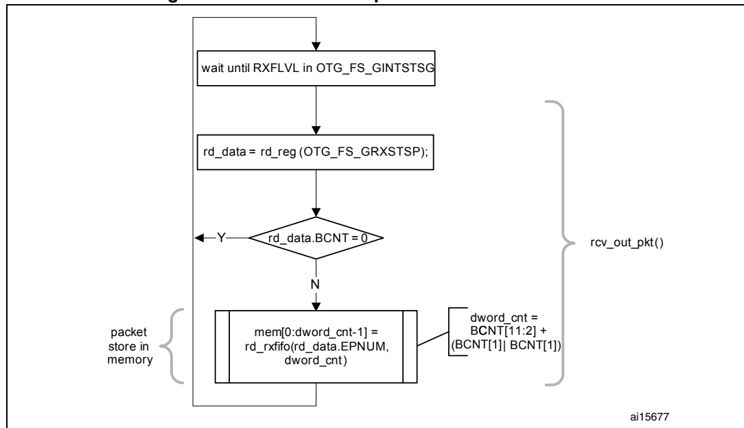
Figure 423. Receive FIFO packet read in slave mode
