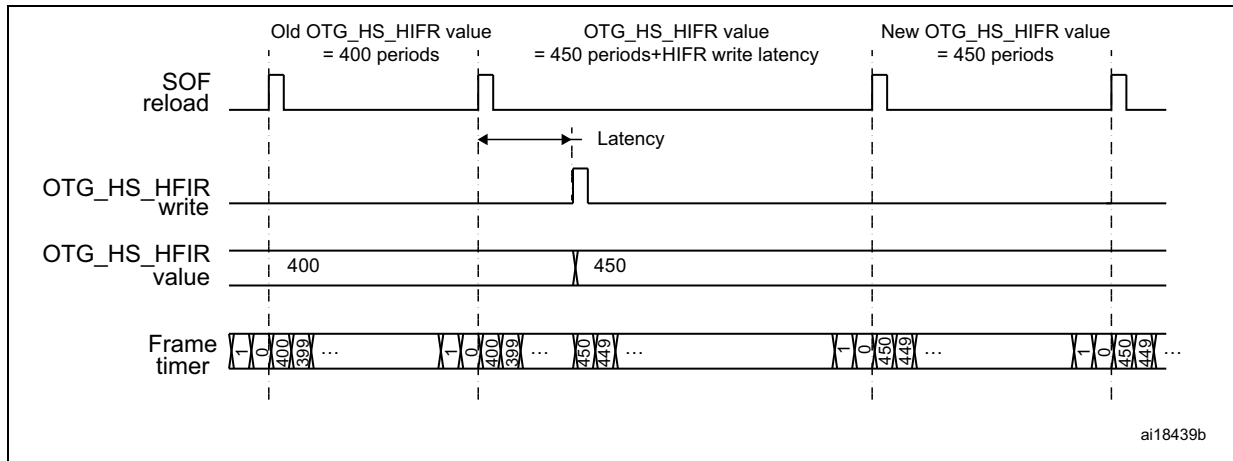
Figure 410. Updating OTG_HS_HFIR dynamically
