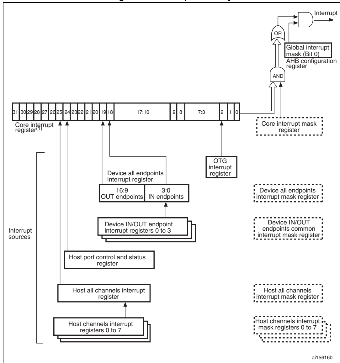
Figure 393. Interrupt hierarchy
