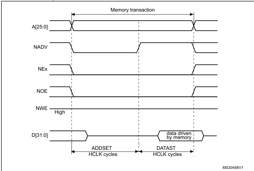
Figure 459. Mode2 and mode B read access waveforms
