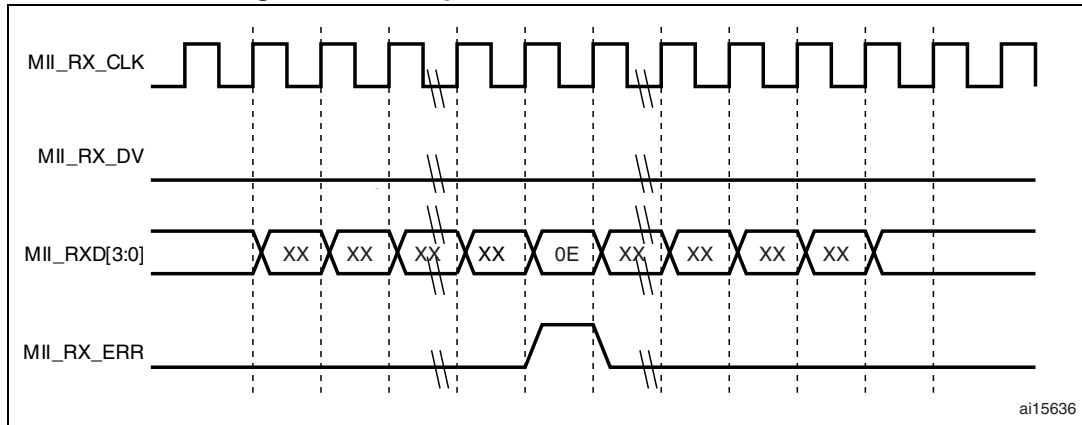
Figure 368. Reception with false carrier indication
