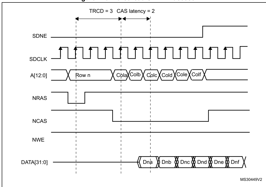
Figure 476. Burst read SDRAM access
