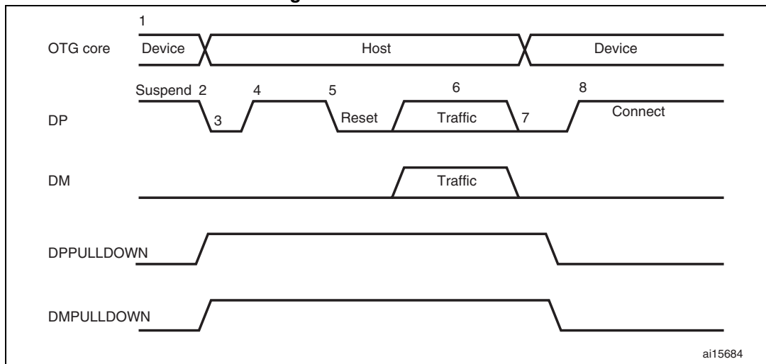
Figure 408. B-device HNP
