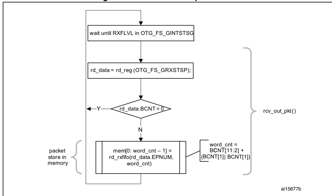
Figure 401. Receive FIFO packet read
