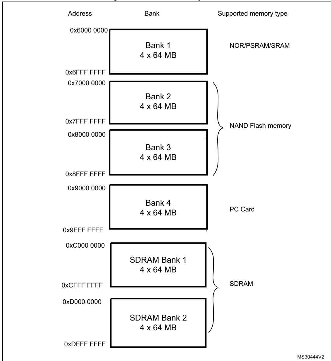
Figure 454. FMC memory banks
