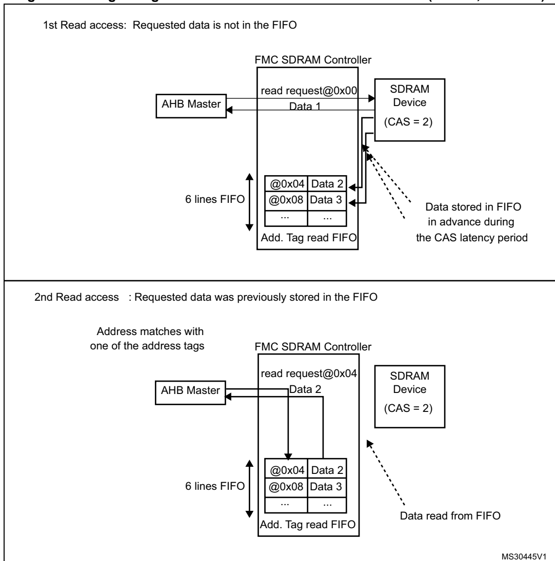
Figure 477. Logic diagram of Read access with RBURST bit set (CAS=2, RPIPE=0)
