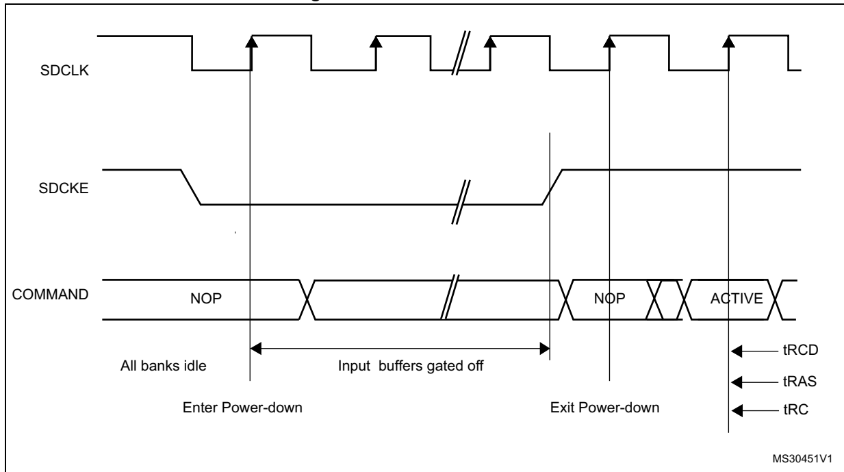
Figure 481. Power-down mode
