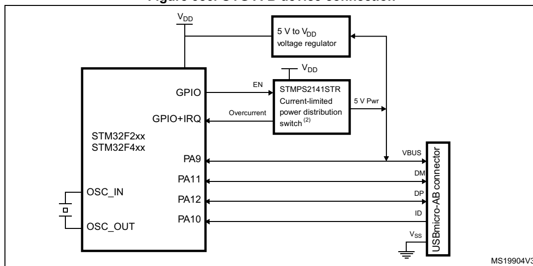
Figure 386. OTG A-B device connection
