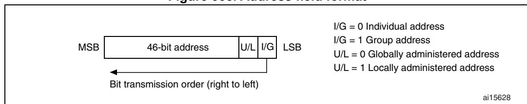
Figure 358. Address field format
