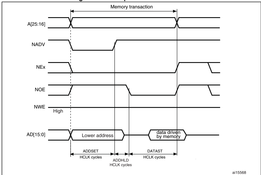
Figure 444. Multiplexed read accesses
