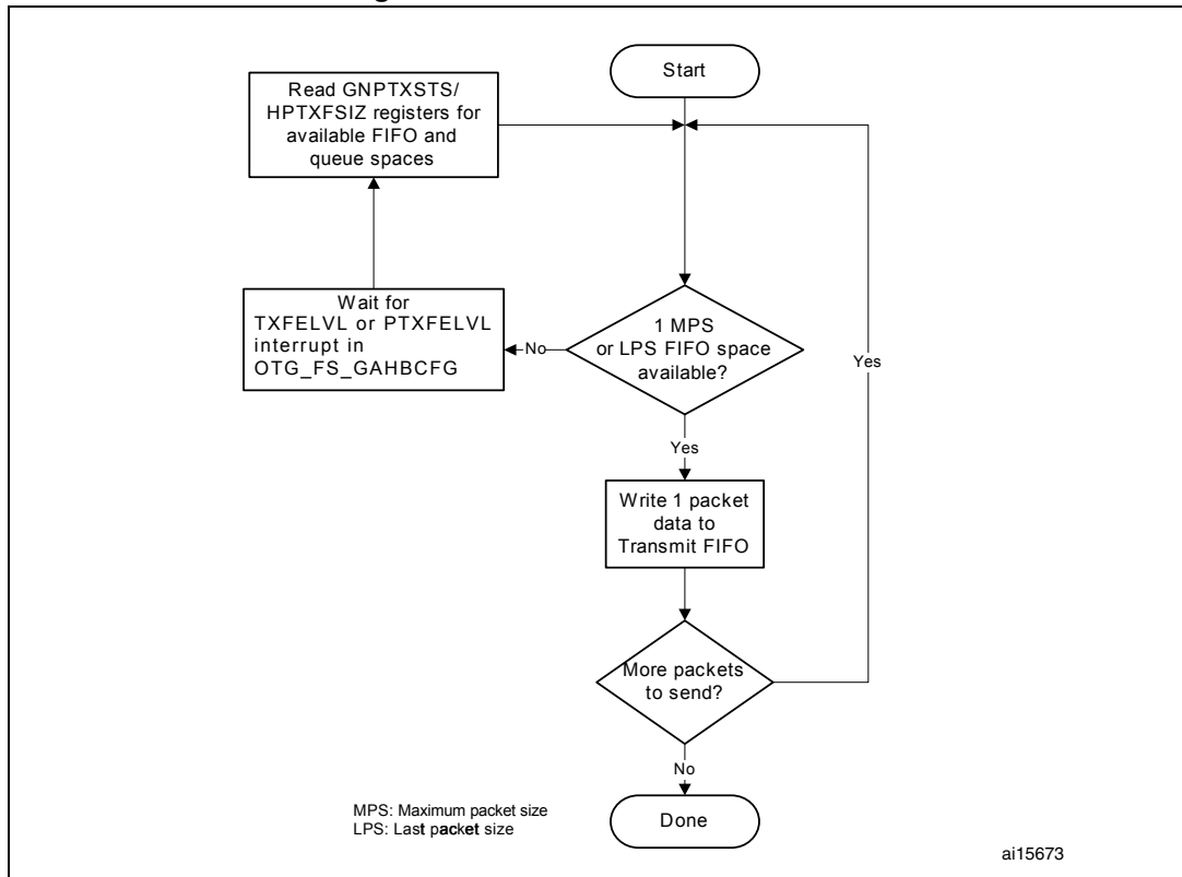
Figure 413. Transmit FIFO write task
