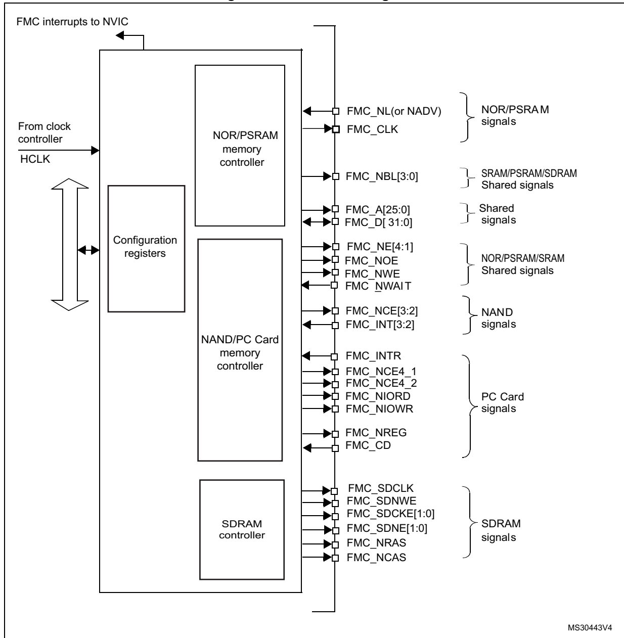
Figure 453. FMC block diagram
