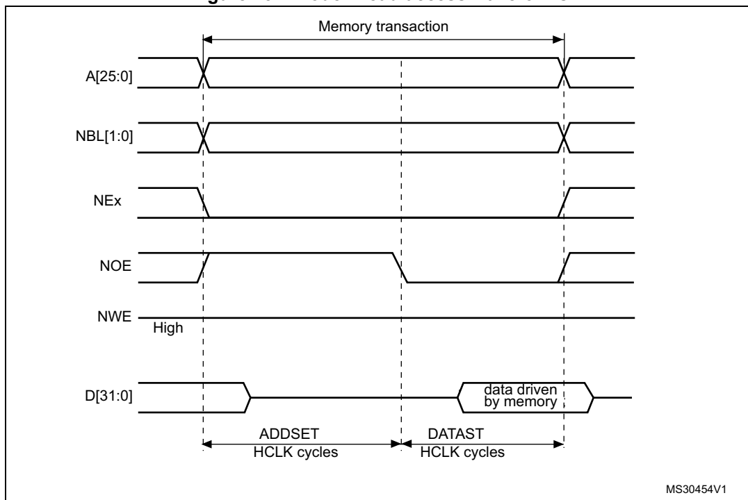
Figure 457. ModeA read access waveforms
