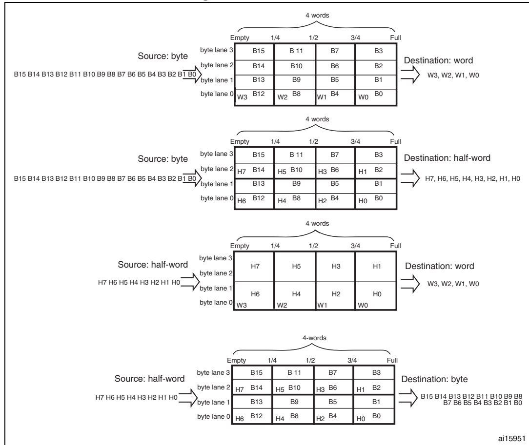
Figure 39. FIFO structure
