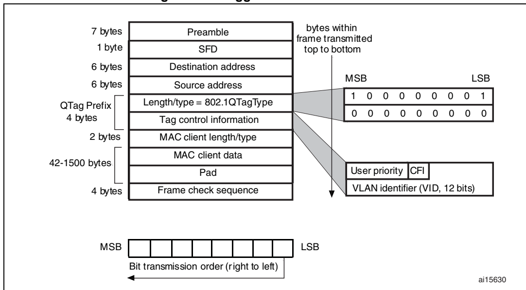
Figure 360. Tagged MAC frame format
