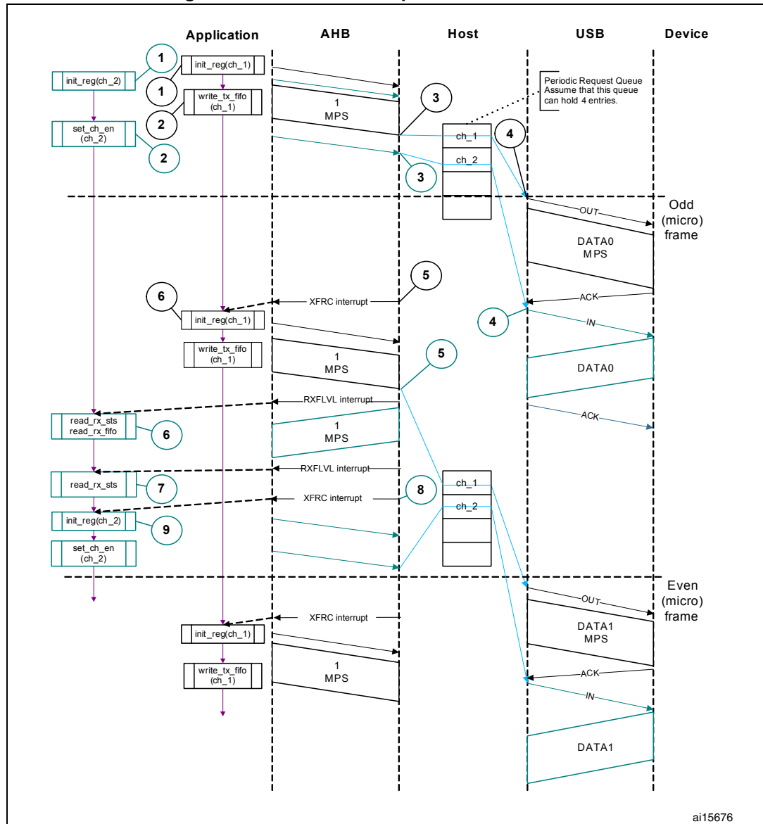
Figure 399. Normal interrupt OUT/IN transactions
