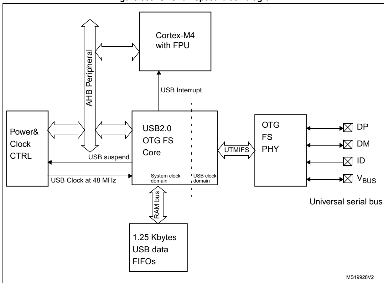
Figure 385. OTG full-speed block diagram
