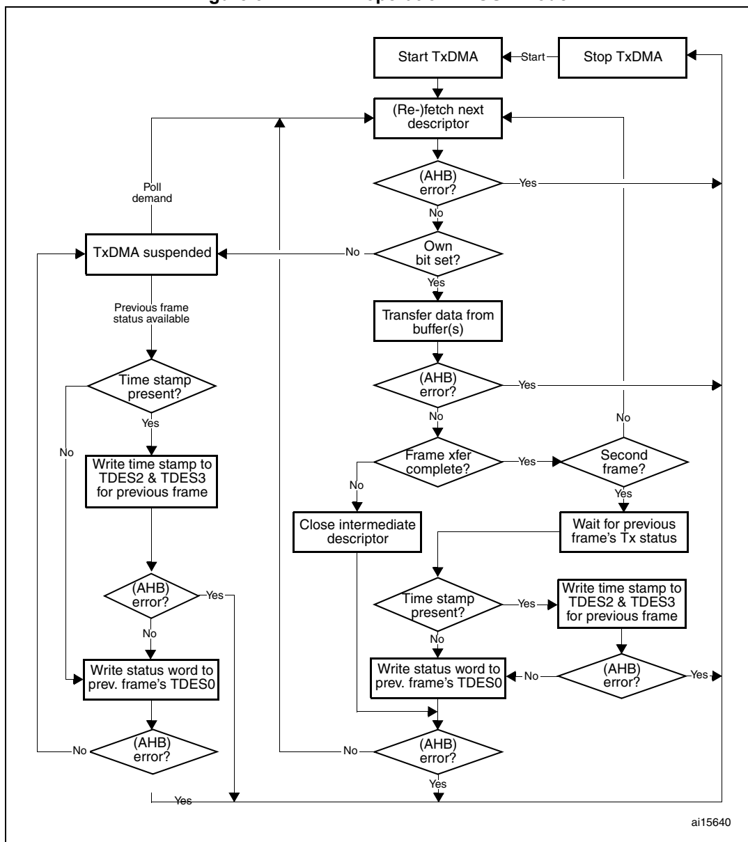
Figure 377. TxDMA operation in OSF mode
