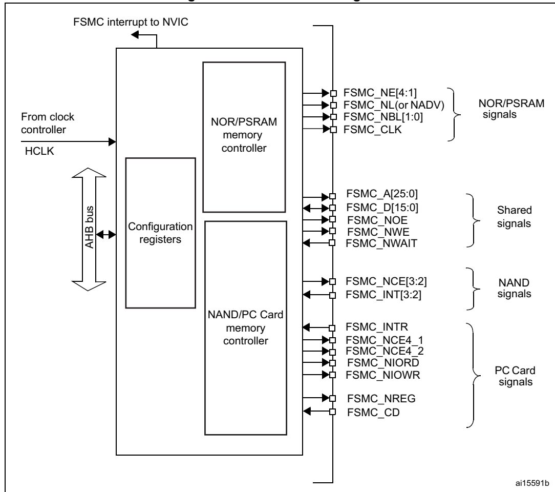
Figure 431. FSMC block diagram
