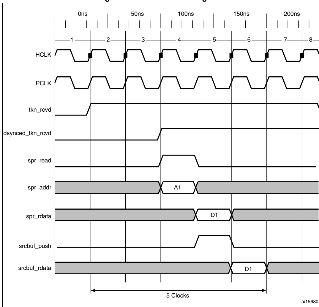
Figure 404. TRDT max timing case
