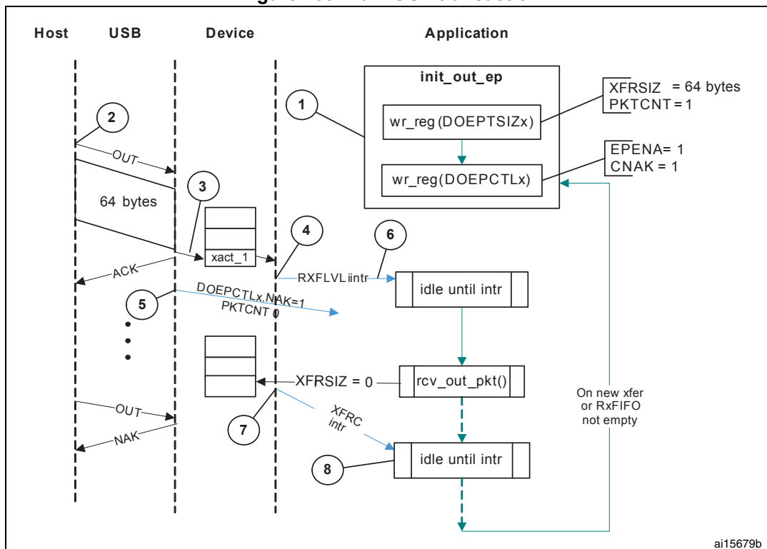
Figure 403. Bulk OUT transaction
