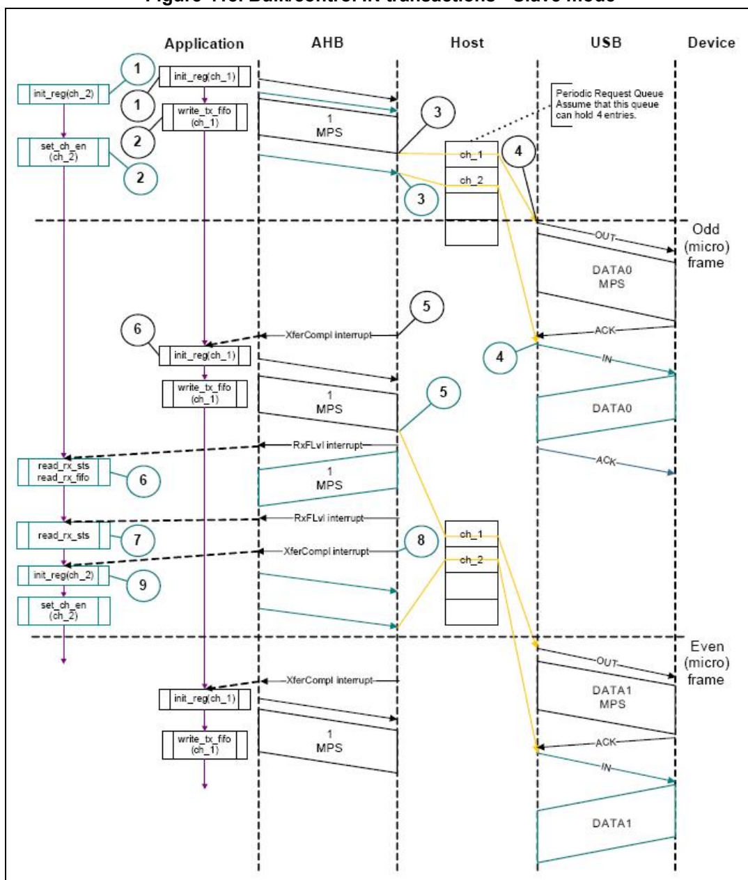
Figure 418. Bulk/control IN transactions - Slave mode
