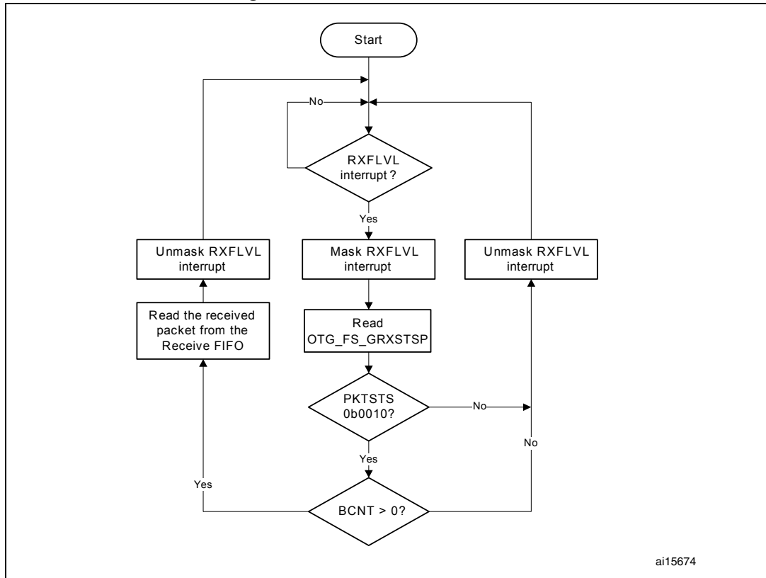
Figure 414. Receive FIFO read task
