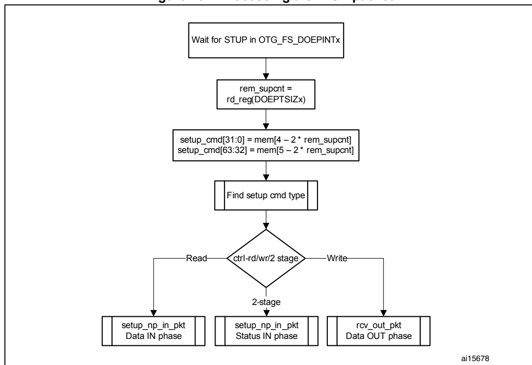
Figure 402. Processing a SETUP packet
