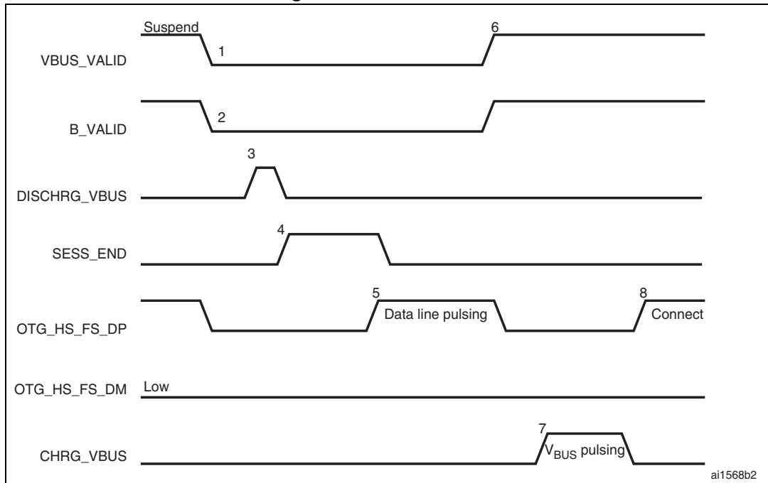
Figure 428. B-device SRP
