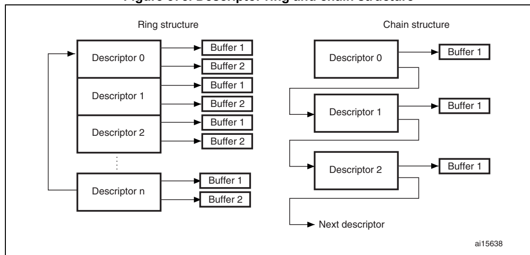
Figure 375. Descriptor ring and chain structure
