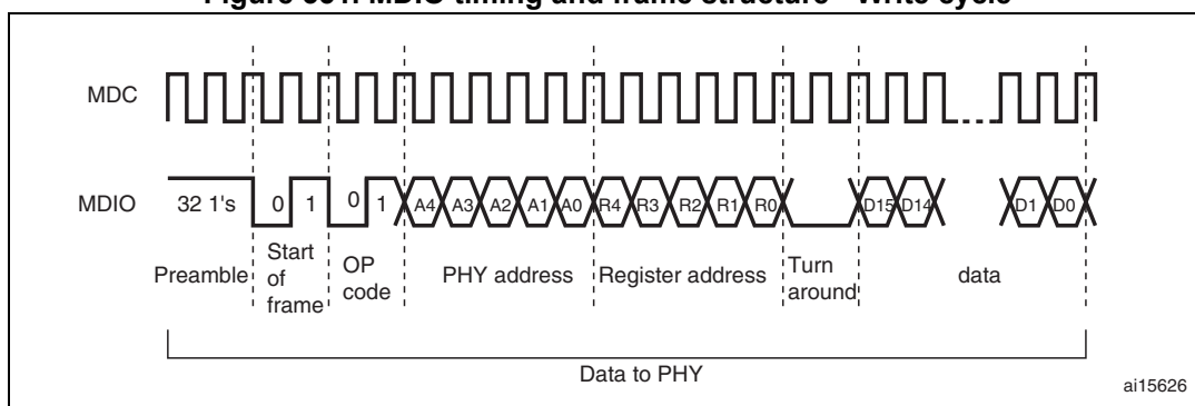
Figure 351. MDIO timing and frame structure - Write cycle
