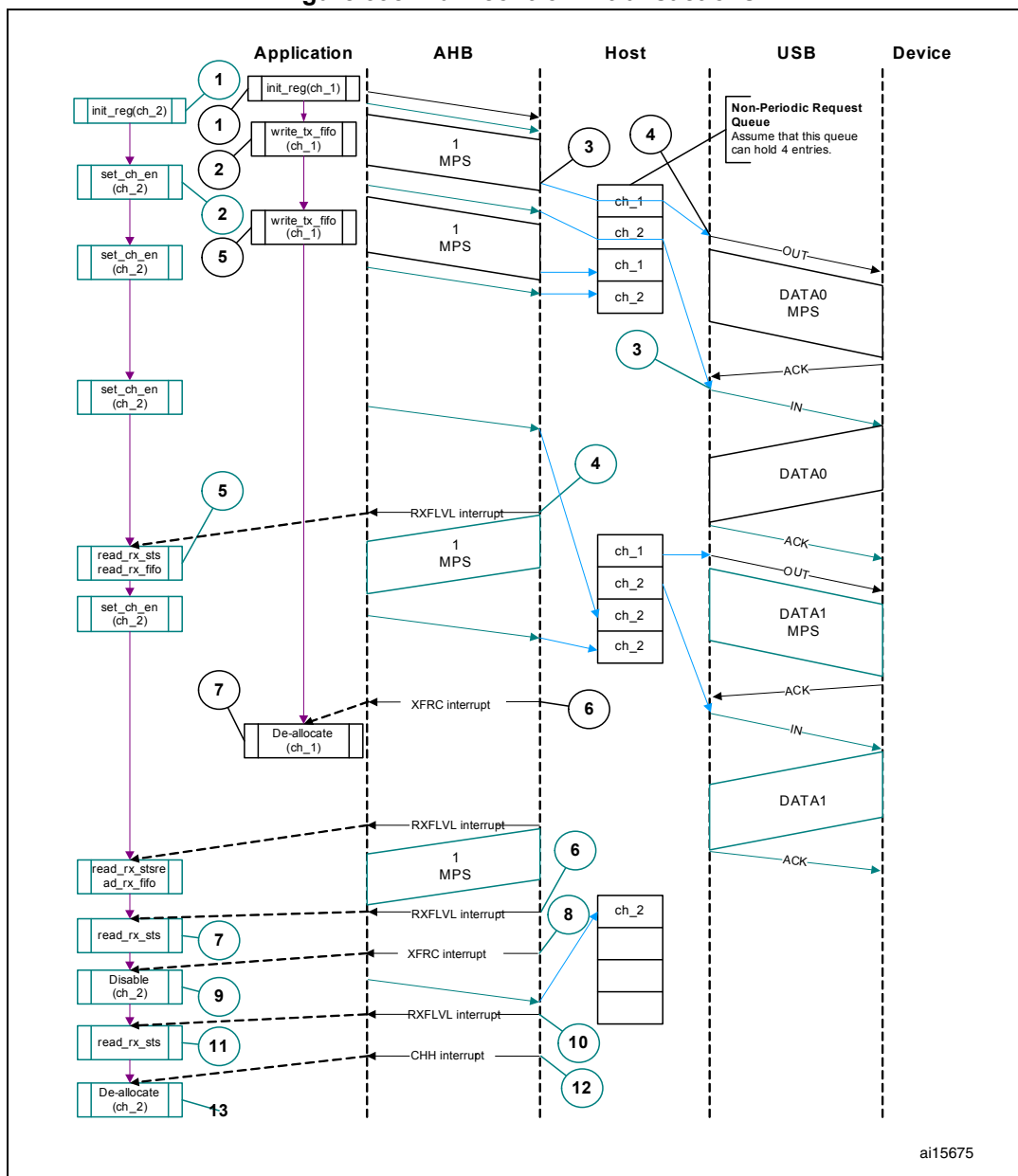
Figure 398. Bulk/control IN transactions
