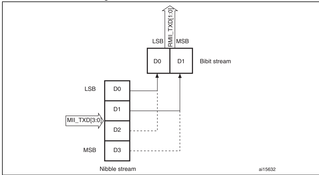
Figure 361. Transmission bit order
