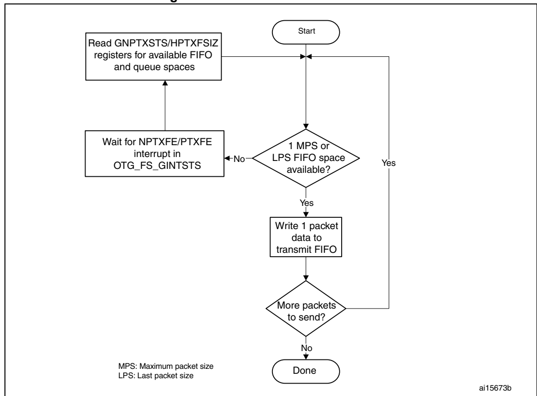
Figure 395. Transmit FIFO write task
