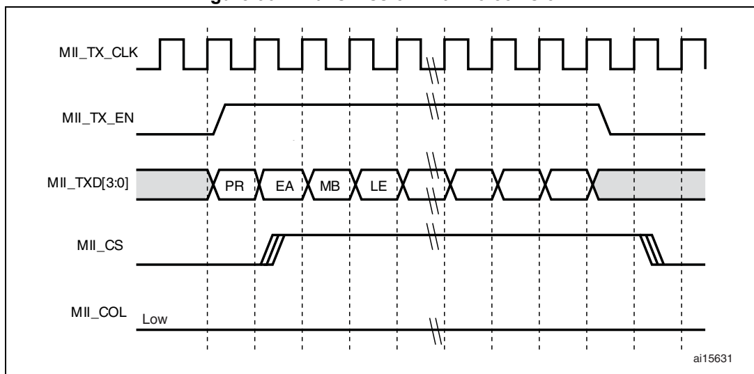
Figure 362. Transmission with no collision
