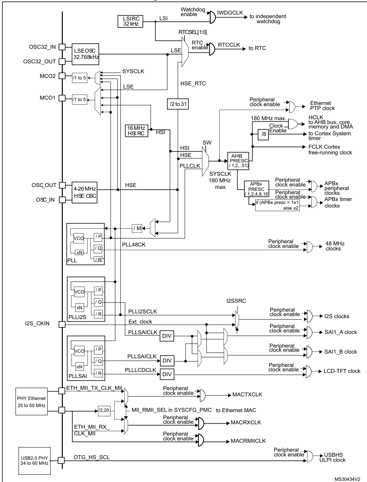
Figure 16. Clock tree
