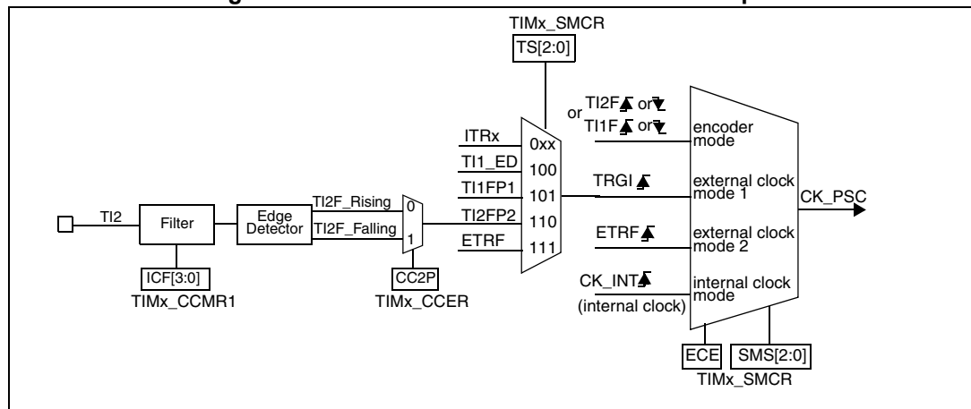
Figure 108. TI2 external clock connection example
