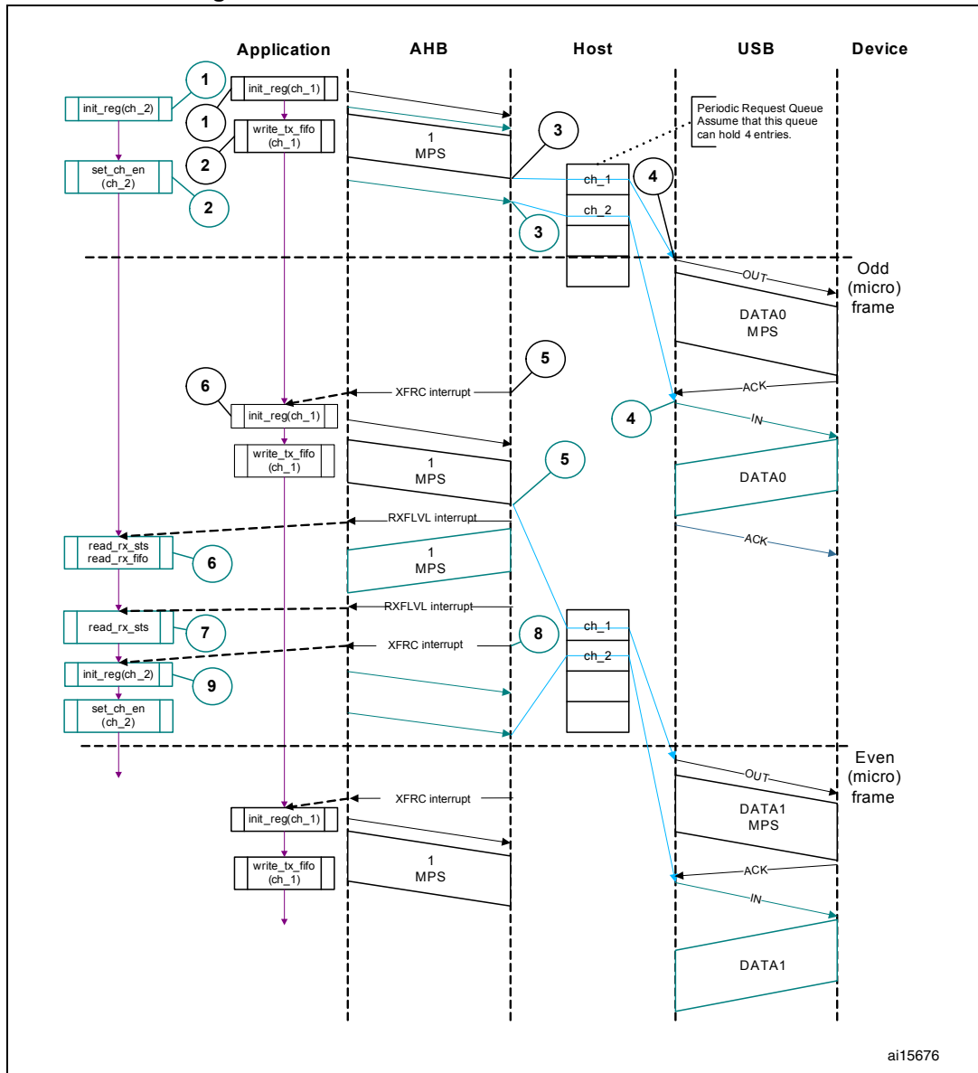
Figure 400. Normal isochronous OUT/IN transactions
