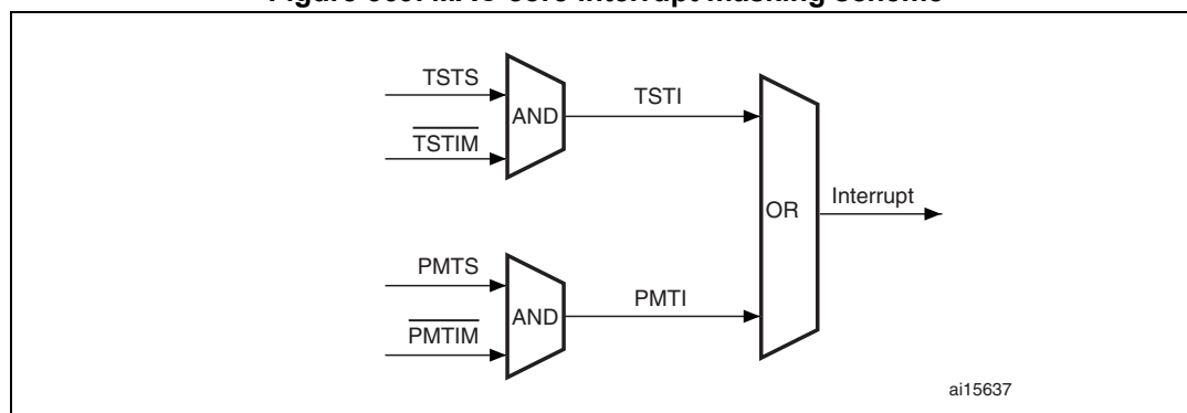
Figure 369. MAC core interrupt masking scheme
