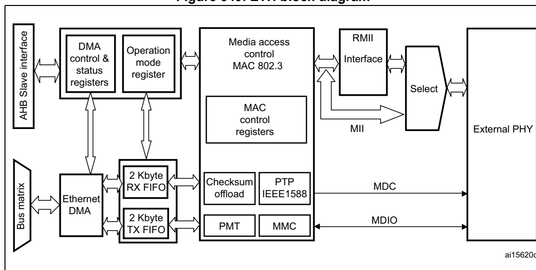
Figure 349. ETH block diagram
