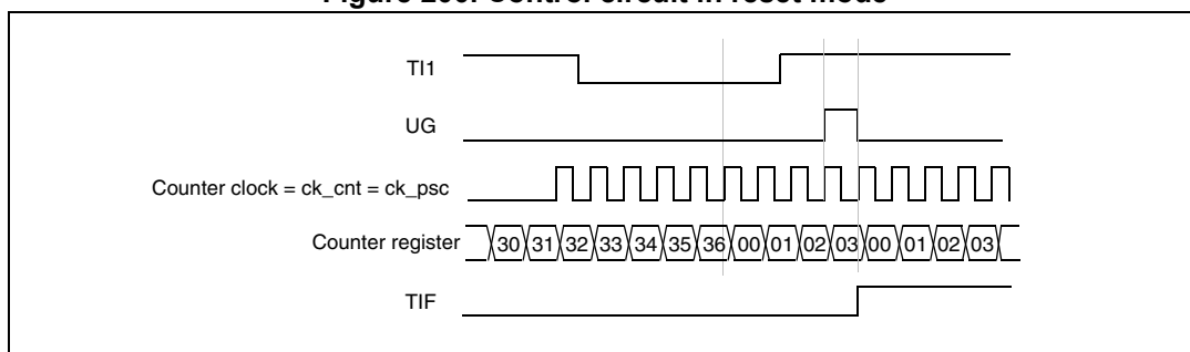
Figure 200. Control circuit in reset mode
