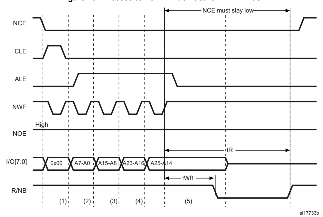
Figure 452. Access to non ‘CE don’t care’ NAND-Flash
