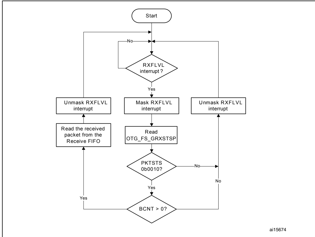
Figure 396. Receive FIFO read task
