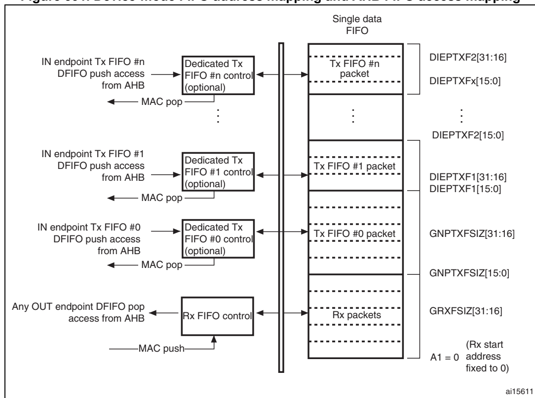
Figure 391. Device-mode FIFO address mapping and AHB FIFO access mapping
