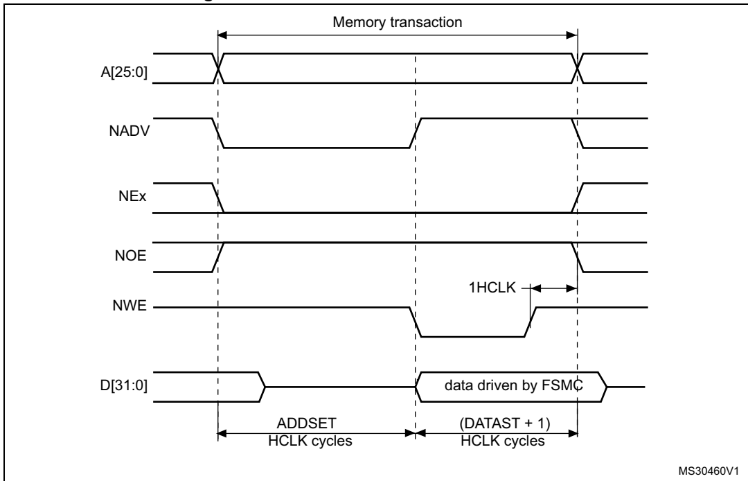
Figure 463. ModeC write access waveforms
