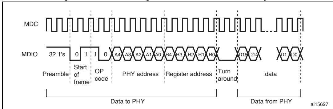
Figure 352. MDIO timing and frame structure - Read cycle
