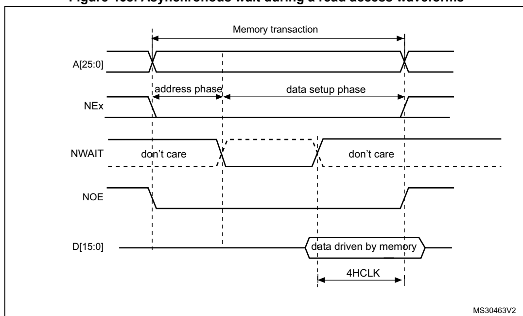
Figure 468. Asynchronous wait during a read access waveforms
