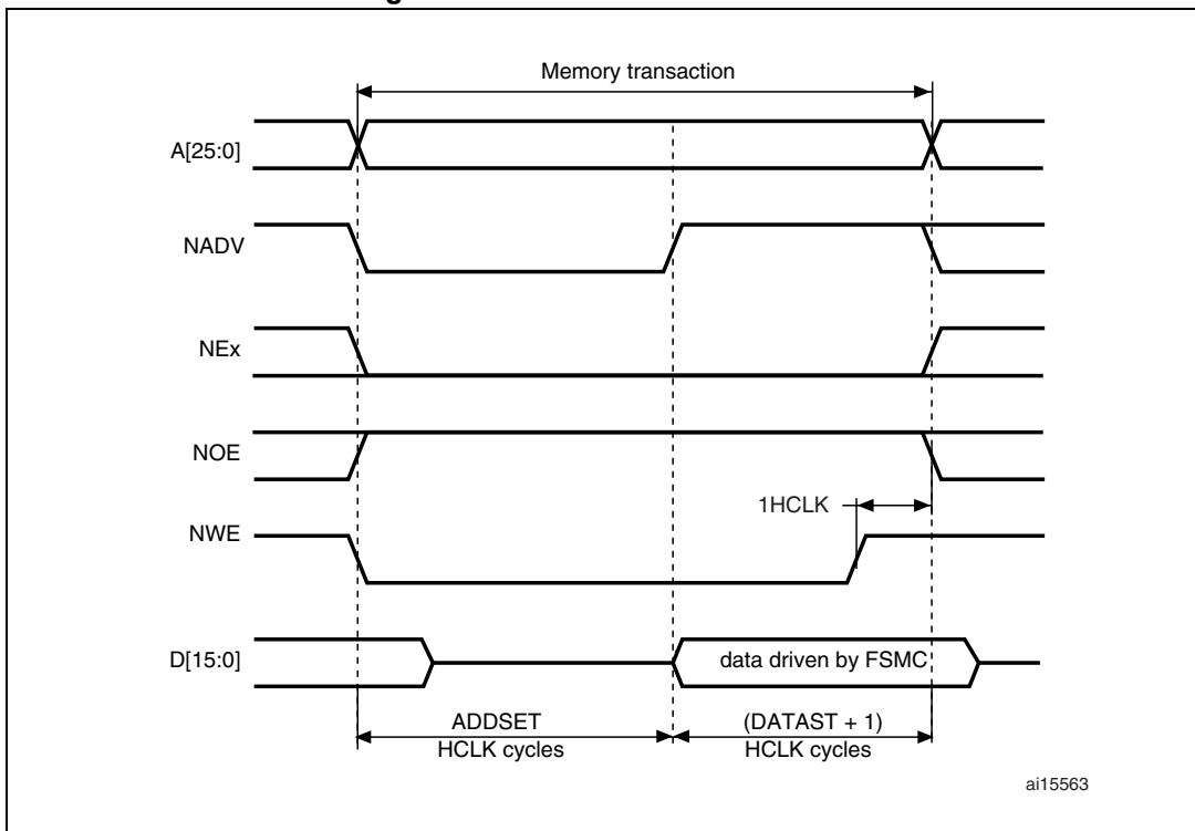
Figure 439. Mode B write accesses
