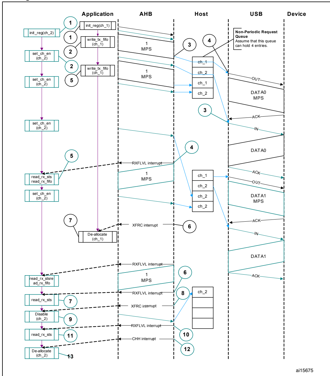
Figure 397. Normal bulk/control OUT/SETUP and bulk/control IN transactions
