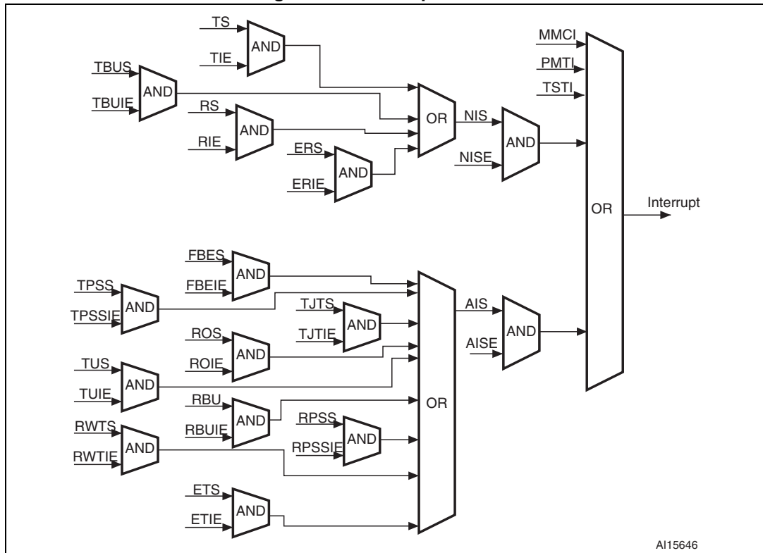
Figure 383. Interrupt scheme
