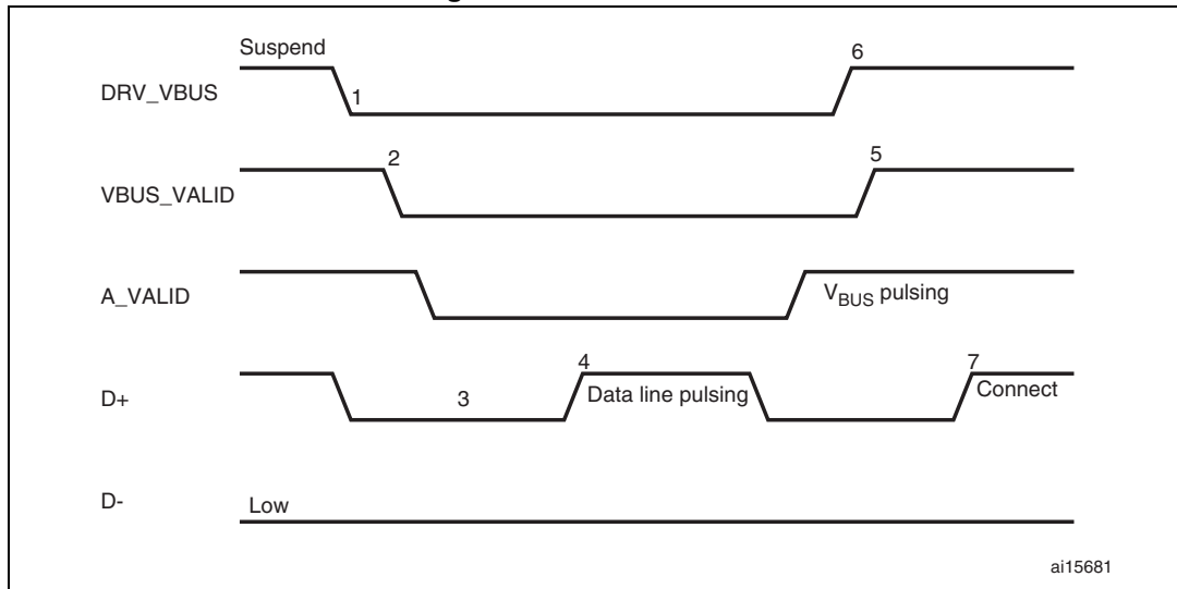
Figure 405. A-device SRP
