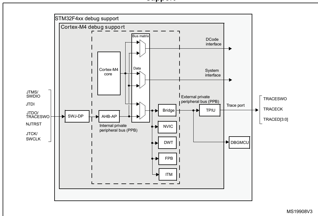
Figure 482. Block diagram of STM32 MCU and Cortex™-M4 with FPU-level debug support
