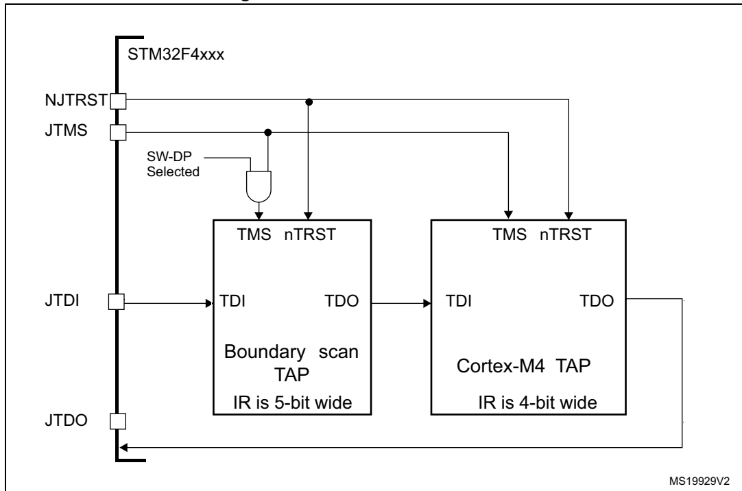
Figure 484. JTAG TAP connections
