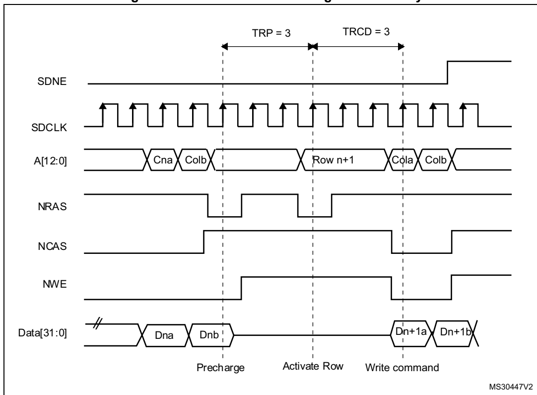
Figure 479. Write access crossing row boundary
