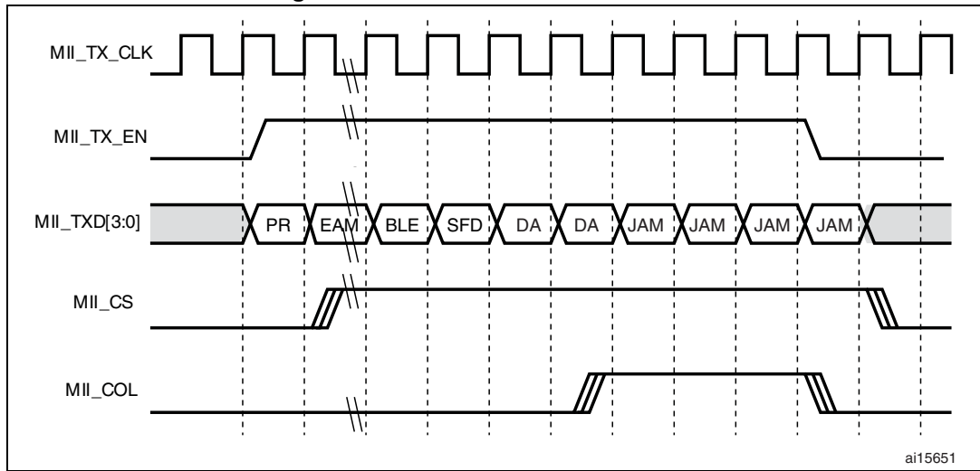
Figure 363. Transmission with collision
