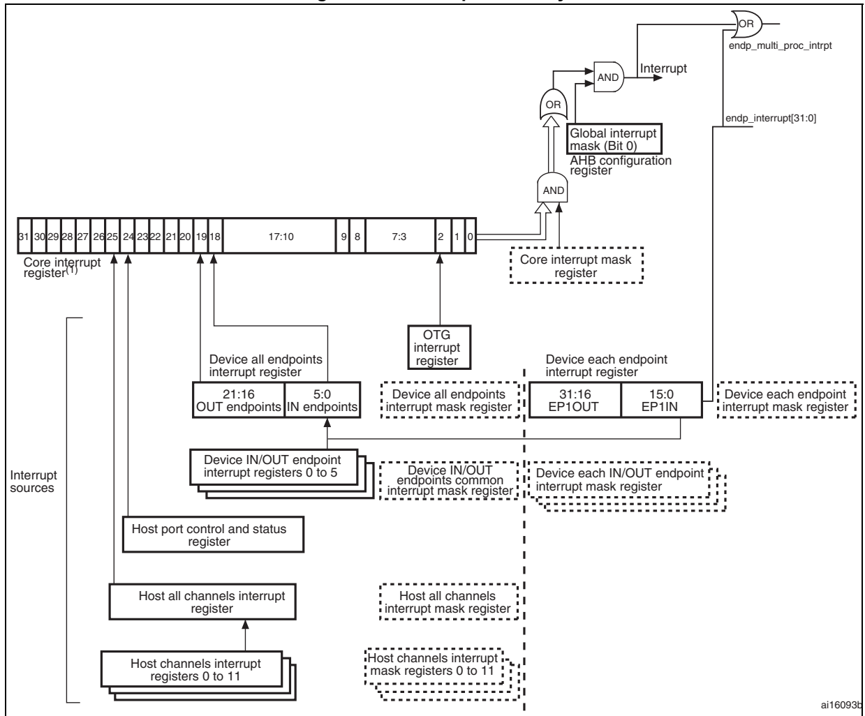
Figure 411. Interrupt hierarchy
