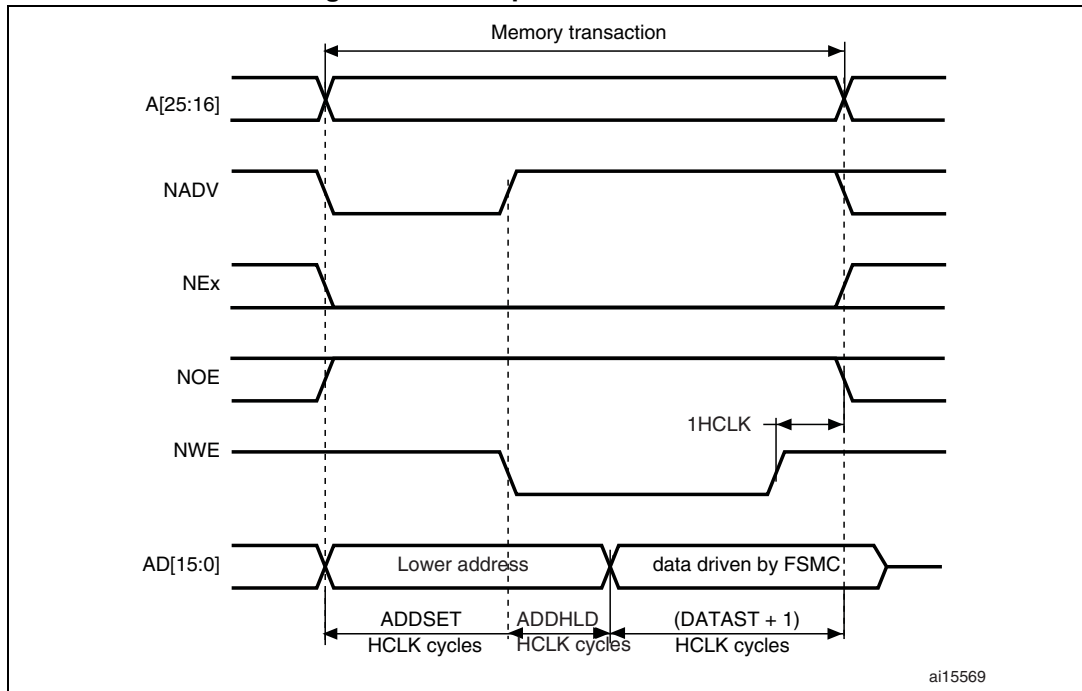
Figure 445. Multiplexed write accesses
