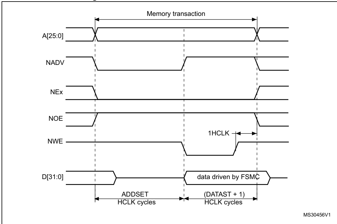
Figure 460. Mode2 write access waveforms
