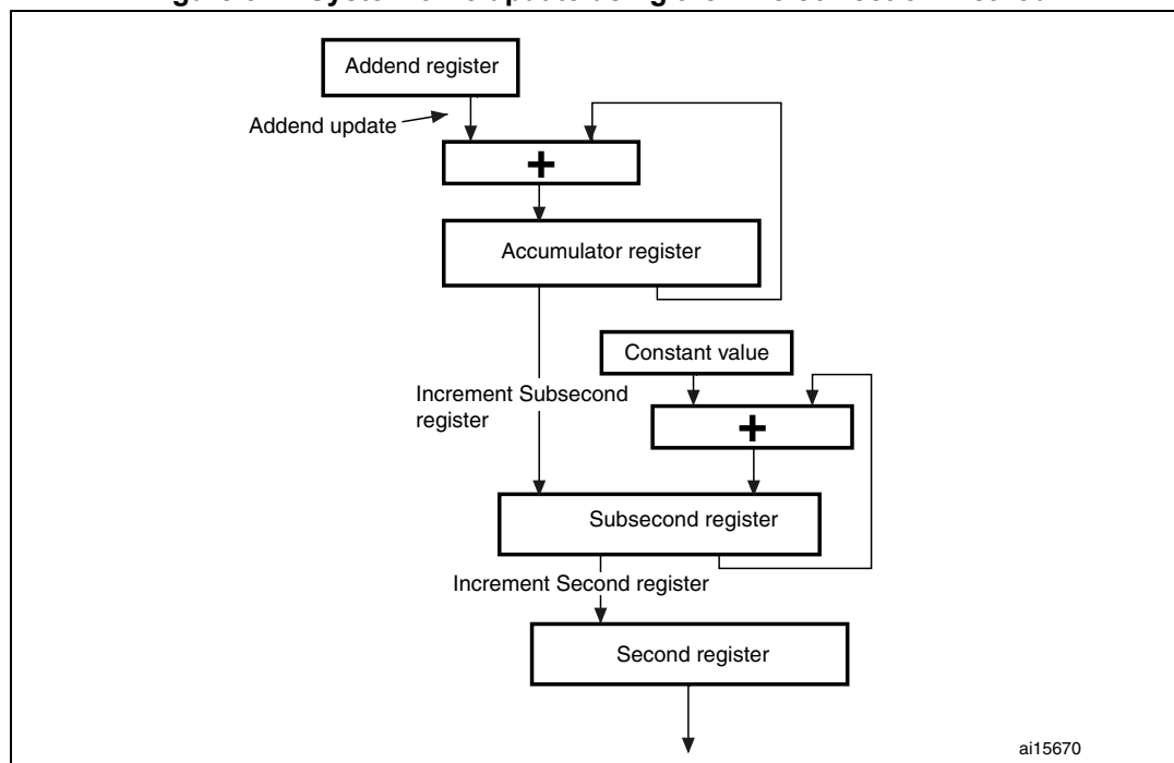
Figure 372. System time update using the Fine correction method
