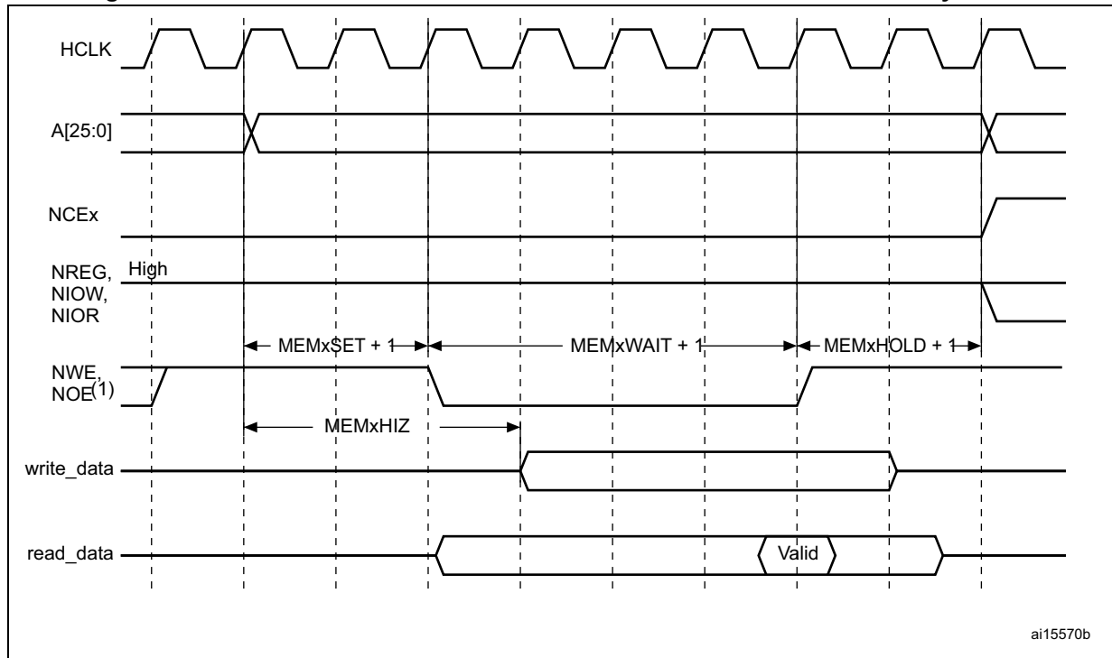
Figure 473. NAND Flash/PC Card controller waveforms for common memory access
