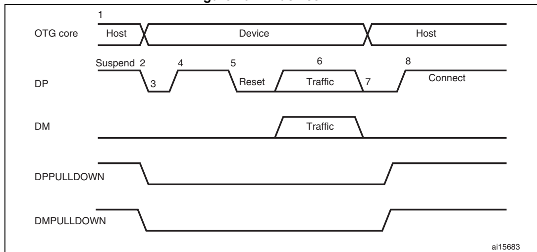
Figure 407. A-device HNP
