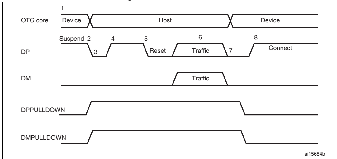
Figure 430. B-device HNP
