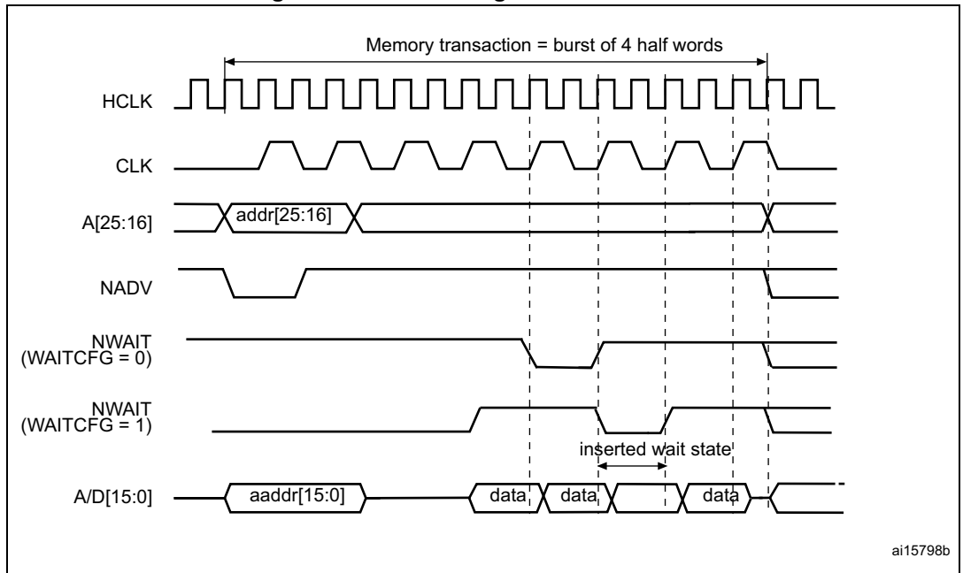
Figure 470. Wait configuration waveforms
