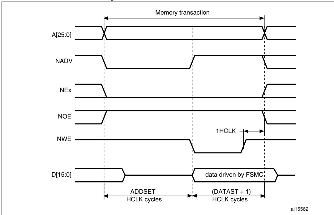
Figure 439. Mode B write accesses
