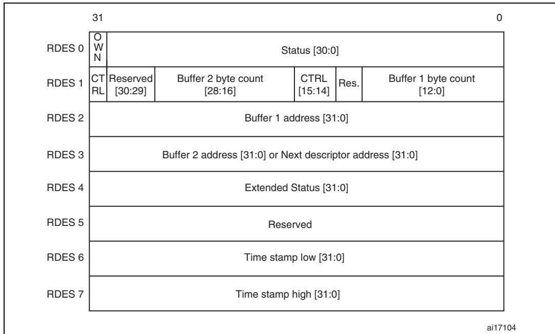
Figure 382. Enhanced receive descriptor field format with IEEE1588 time stamp enabled
