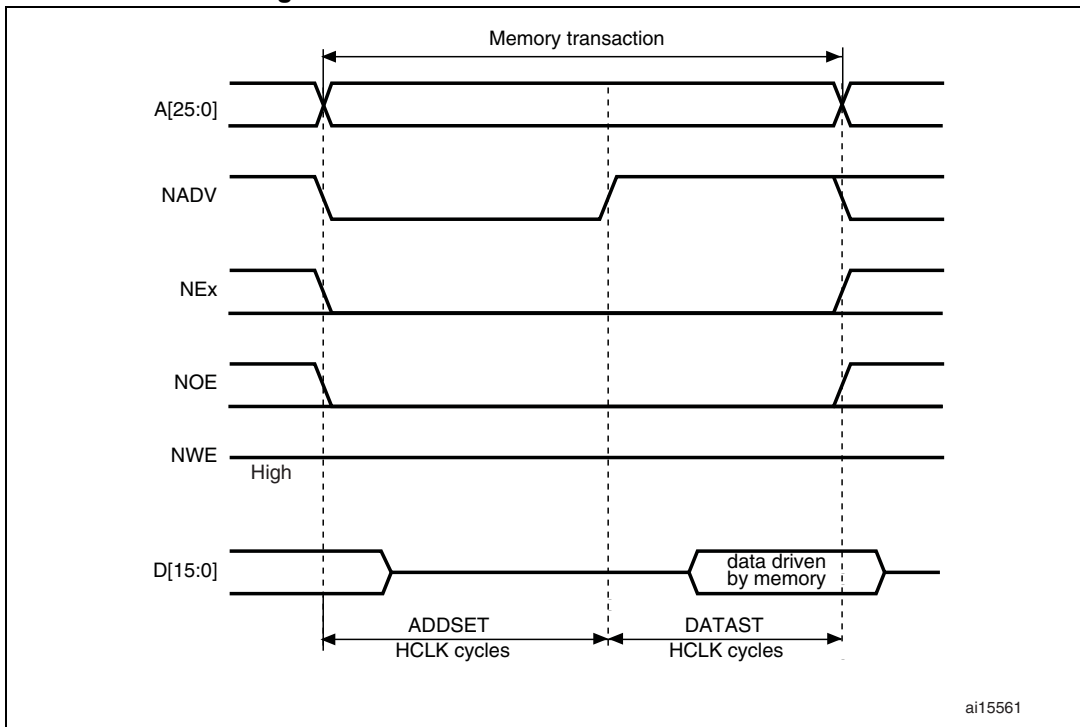
Figure 437. Mode2 and mode B read accesses
