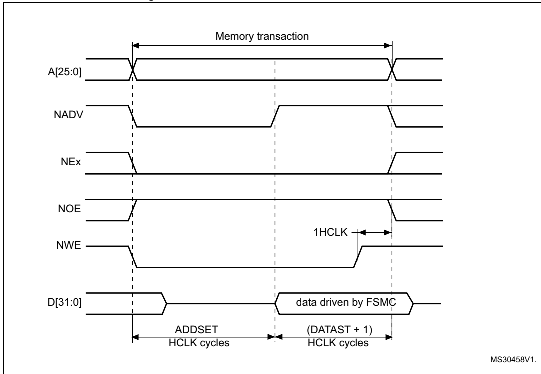
Figure 461. ModeB write access waveforms
