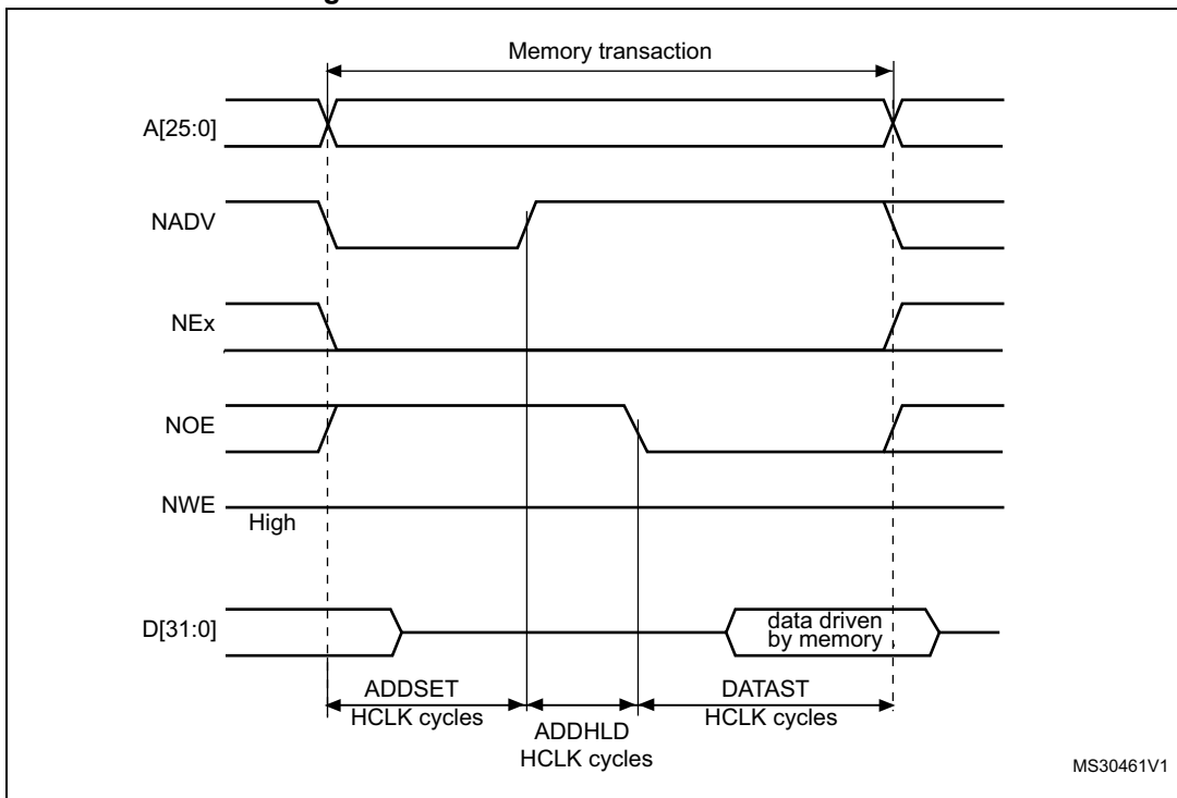
Figure 464. ModeD read access waveforms
