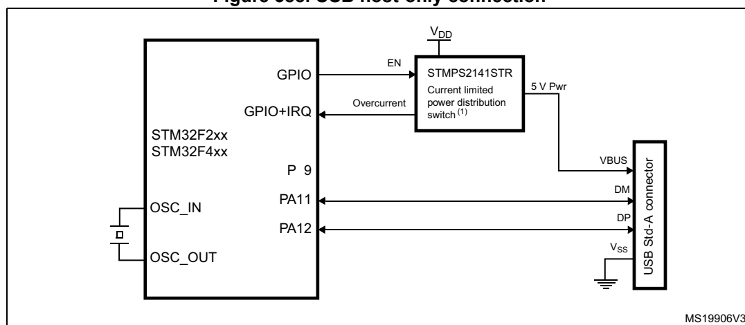
Figure 388. USB host-only connection
