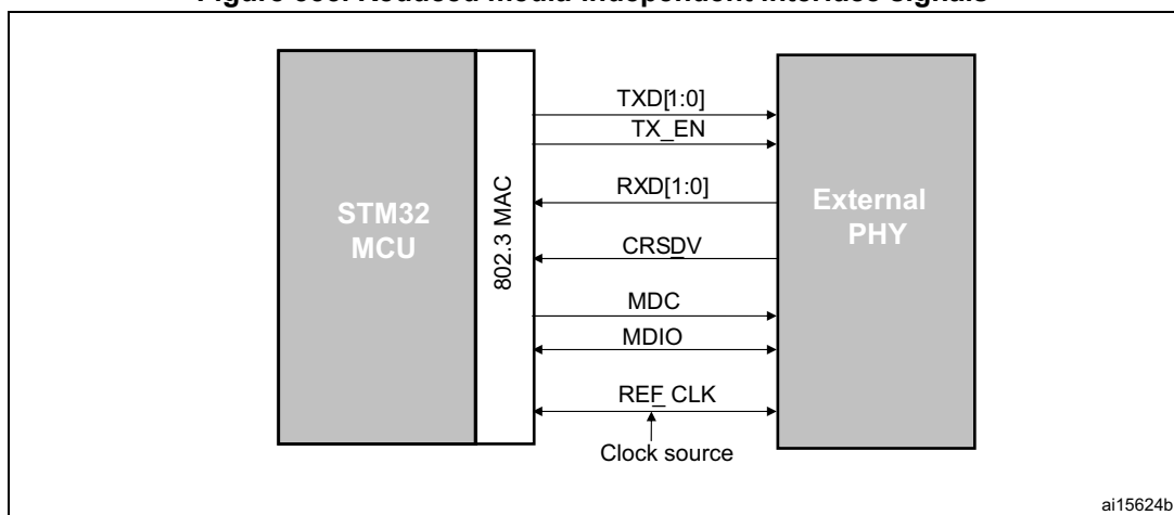
Figure 355. Reduced media-independent interface signals
