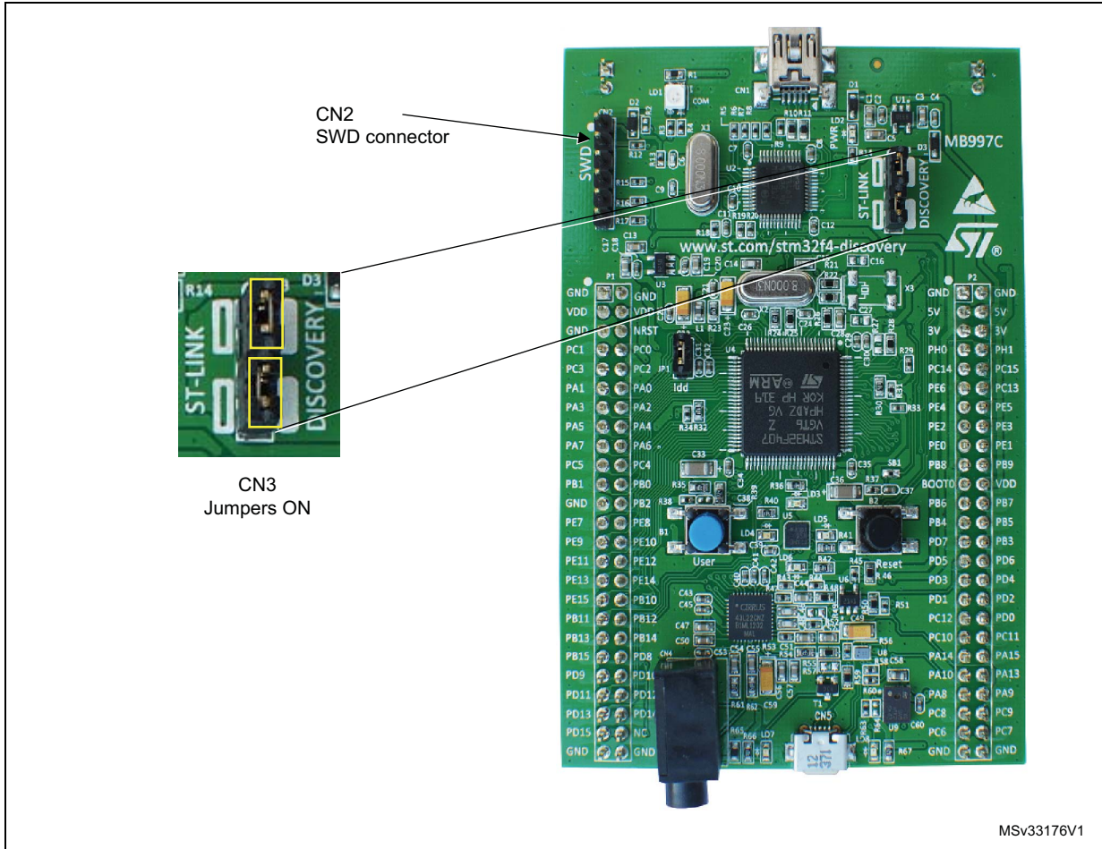
Figure 8. STM32F4DISCOVERY connections image
