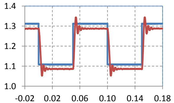
Figure 6: K_p = 50 , K_d = 0 , K_i = 0 ; Proportional gain is high, the actual value (red) is closer to the desired value (blue), but oscillations become visible
